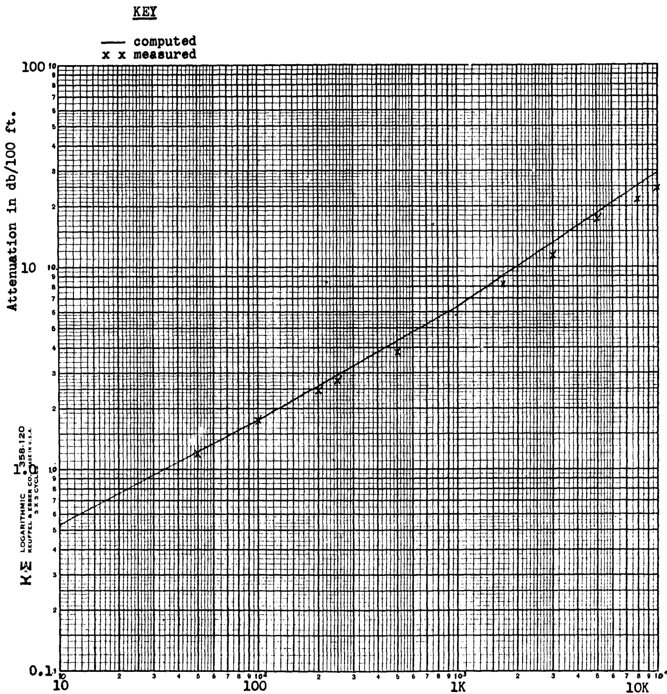
Graph 1.26 - Computed and measured attenuation of sample 30
