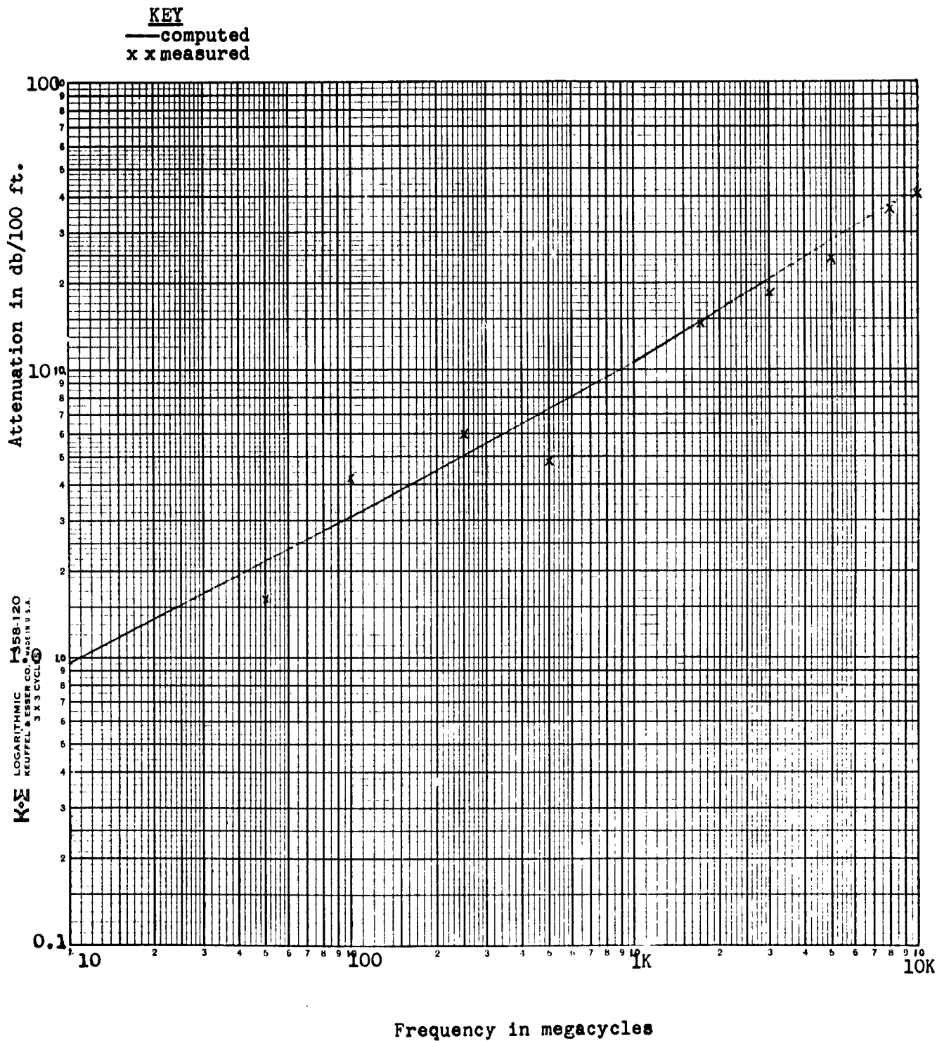
Graph 1.11 - Computed and measured attenuation of sample 12
