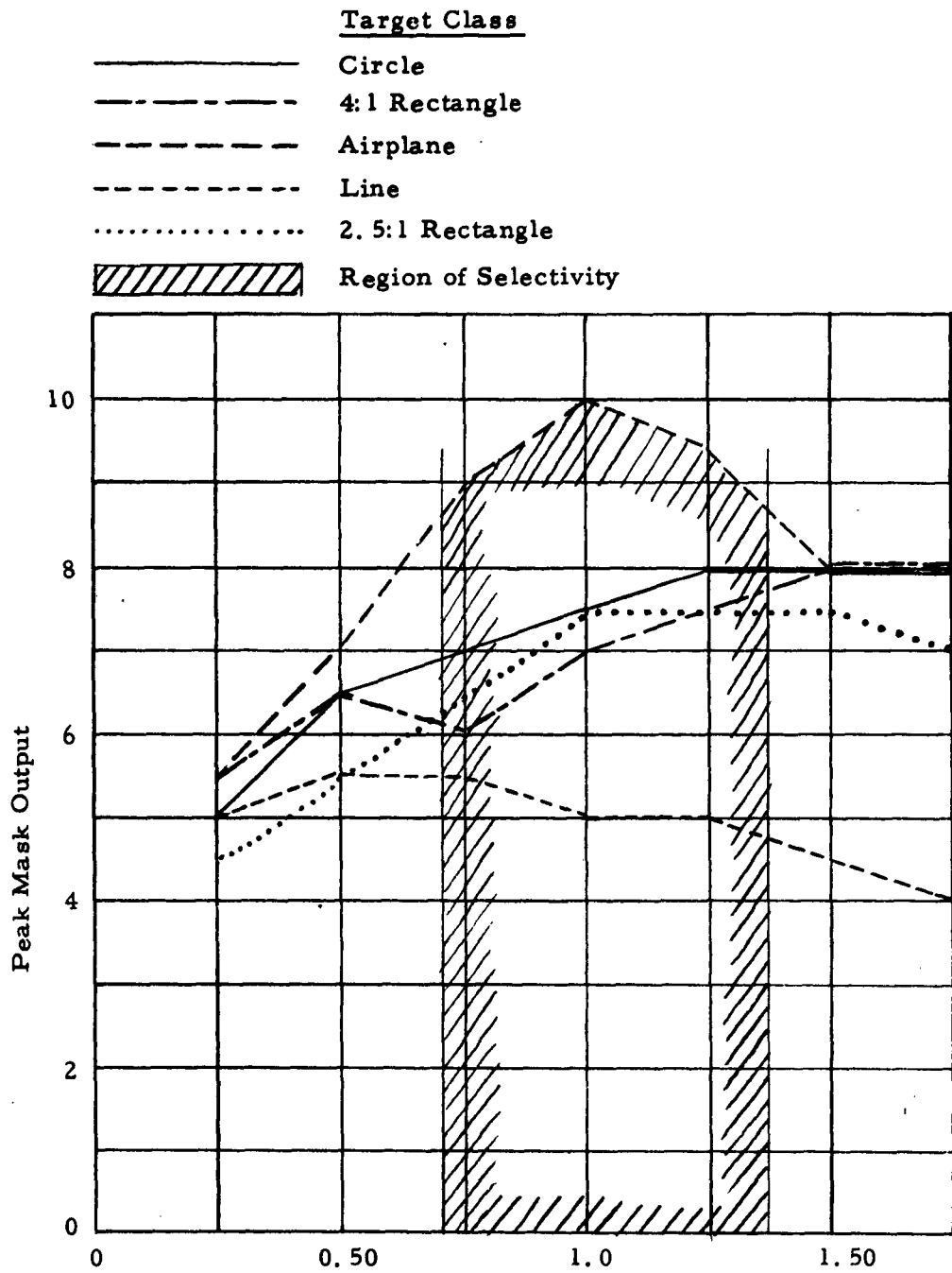
Relative Target Size (Experimental Results) Figure 4.17 - Airplane Mask Output for Five Target Classes
