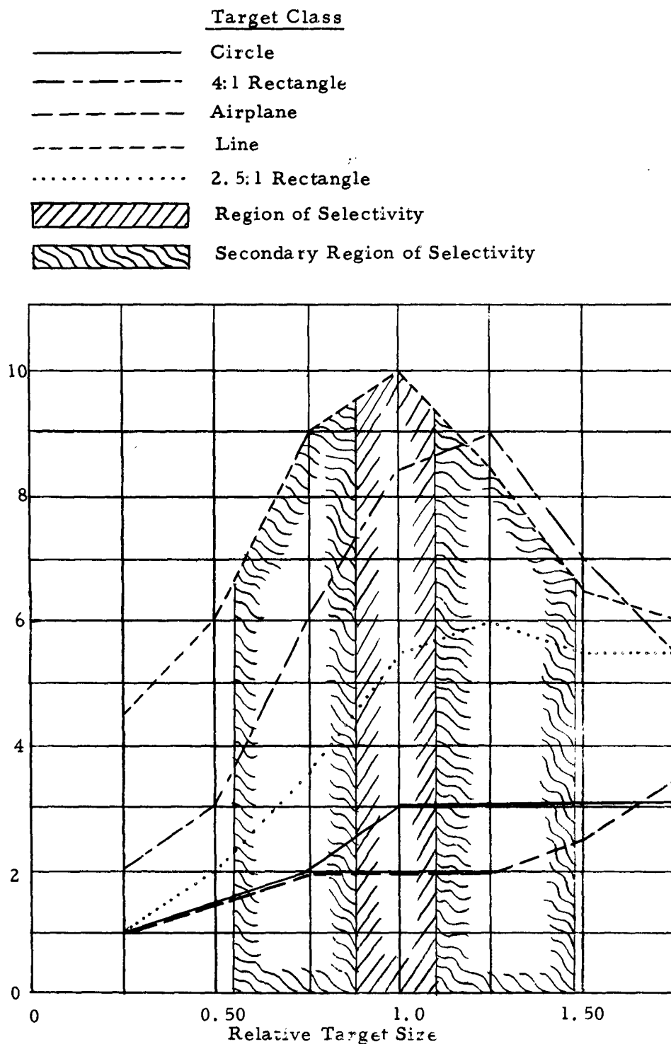
Figure 420 -5:1 Line Mask Output for Five Target Classes
