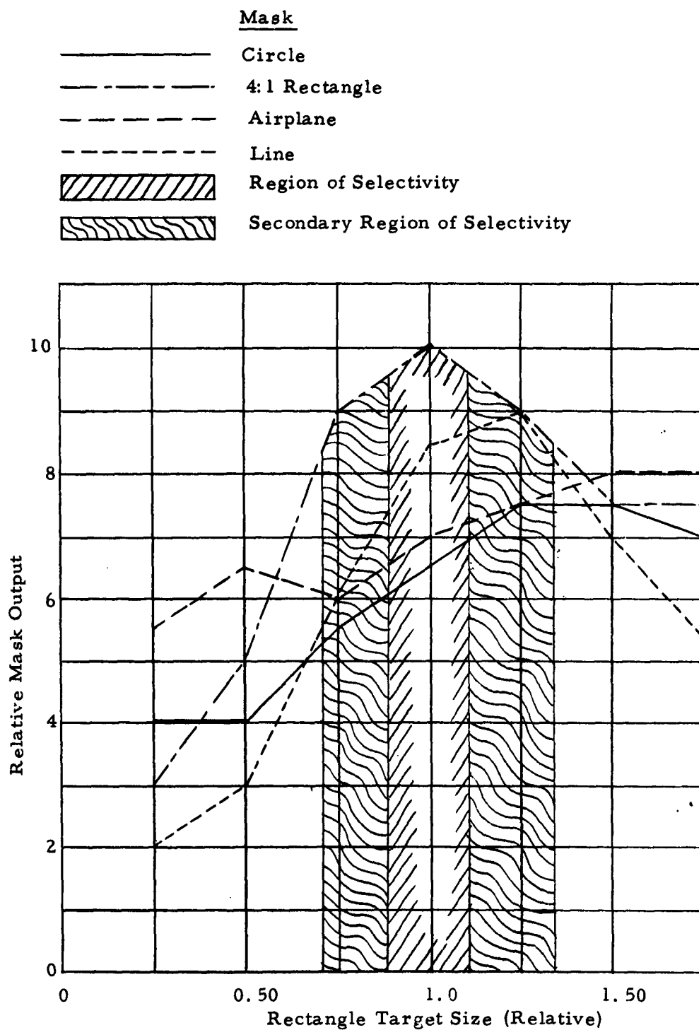
Figure 4.24 - (Experimental Results) Comparative Area-Matching - Target: 4:1 Rectangles
