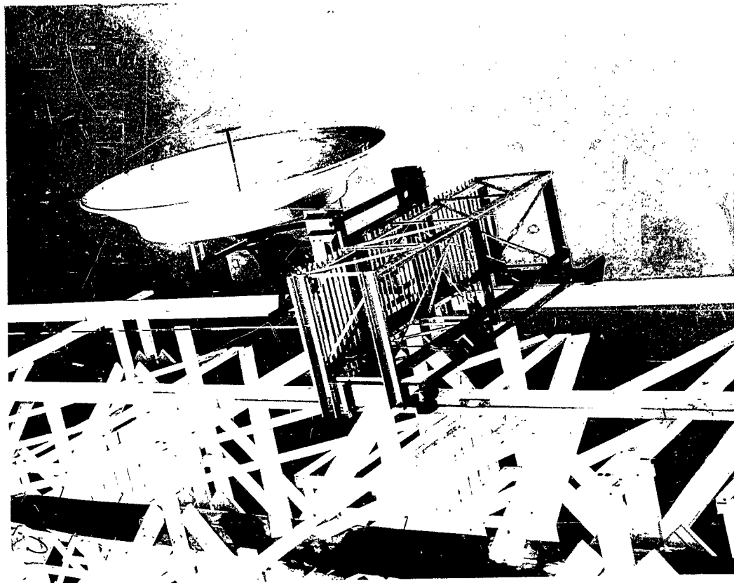
FIG. 11 - TRANSMITTER TOWER POLARIZATION POSITIONER AND TRANSMIT ANTENNA BEING RAISED TO THE TOP OF THE TOWER
