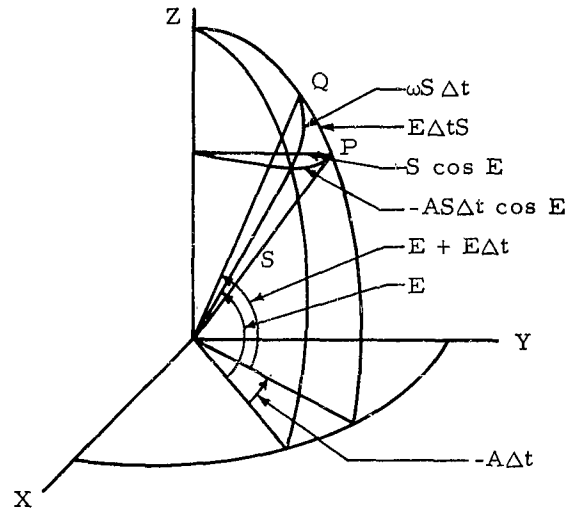
Figure 2. Infinitesimal Rotations
