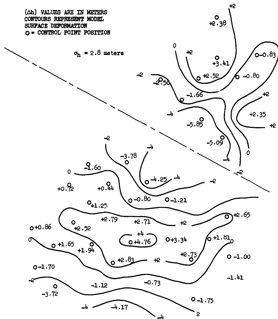
FIGURE 6. RESIDUAL ELEVATION DISTORTION AFTER PARABOLIC ADJUSTMENT (TO REMOVE EFFECTS OF SECOND DEGREE SURFACE DEFORMATION)
