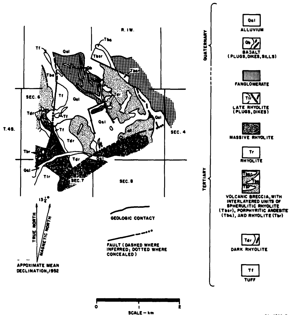
FIG. 3 GEOLOGY SURROUNDING STATION B (After Miesch 3 )
