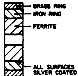
FIG. 3-2. SAMPLE NO. 6513 IRON INSULATED FERRITE
