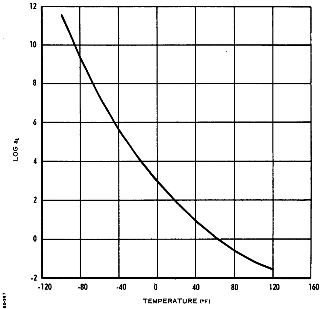
Figure 3-4 Log a_T versus Temperature, Polycarbonate Propellant, Constant Strain Rate Data
