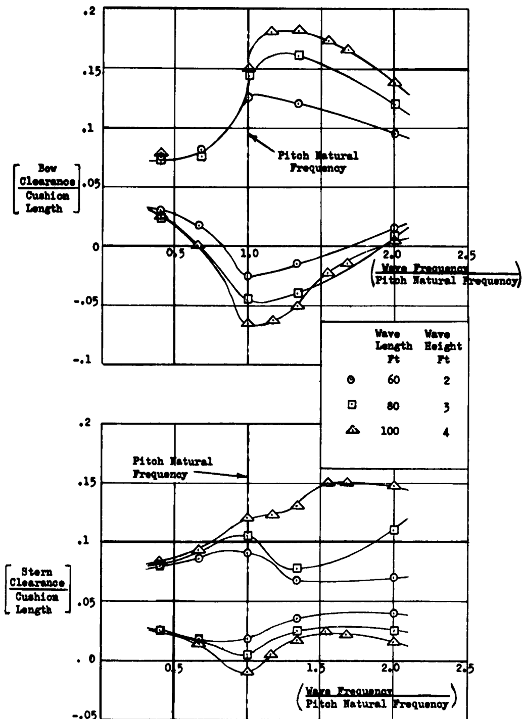
Fig. 39 Wave clearance
