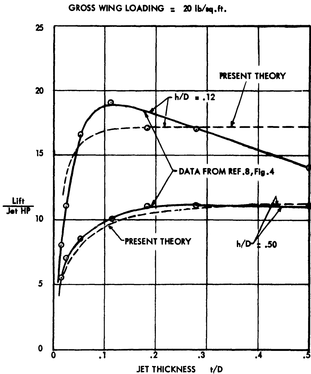
Fig. 51 Variation of lift/jet horsepower with jet thickness
