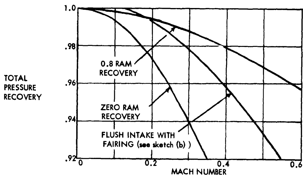
Fig. 59 Intake pressure loss
