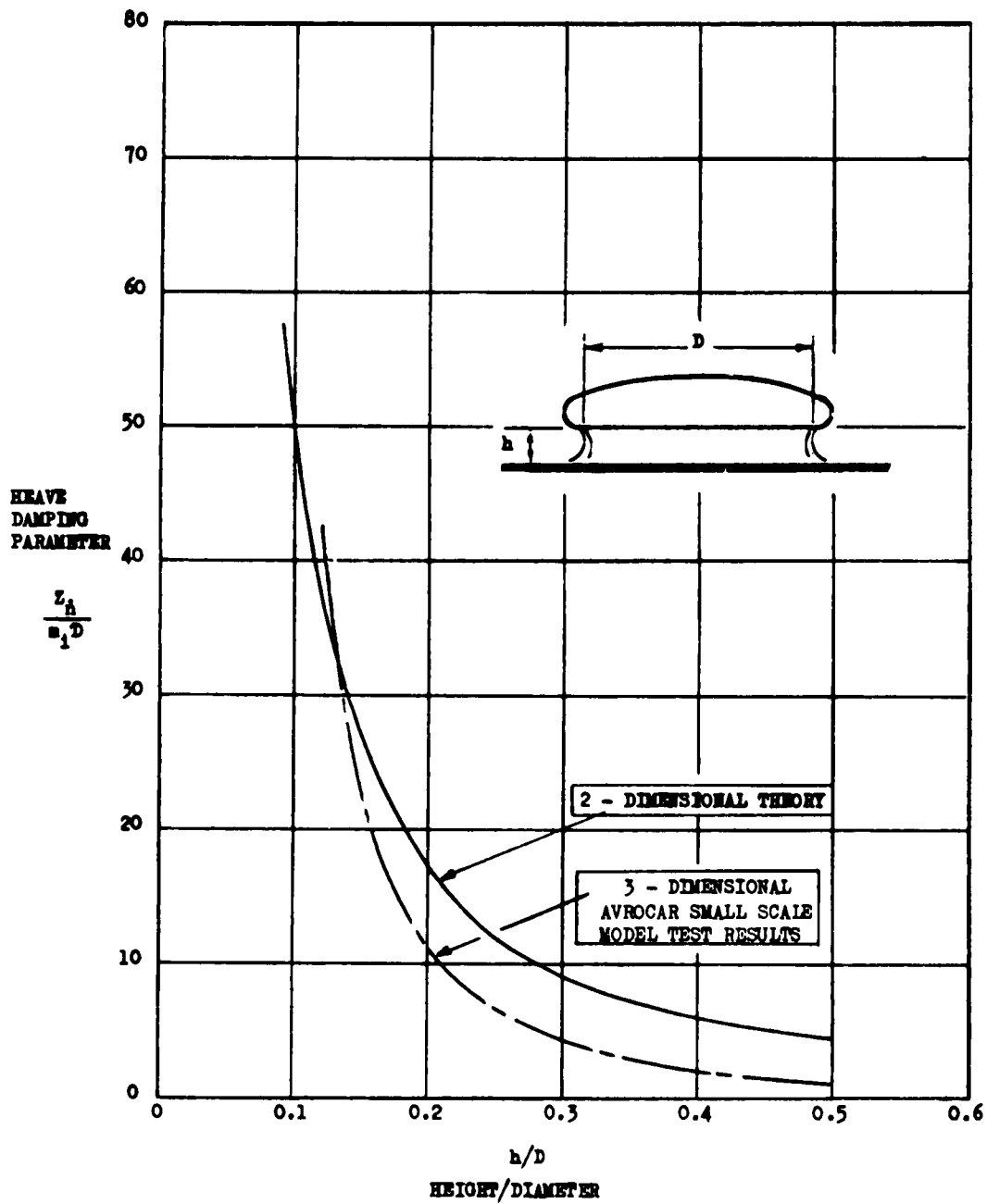
Fig.38 Heave damping
