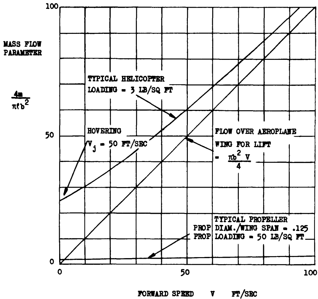
Fig.46 Mass flow variations with forward speed
