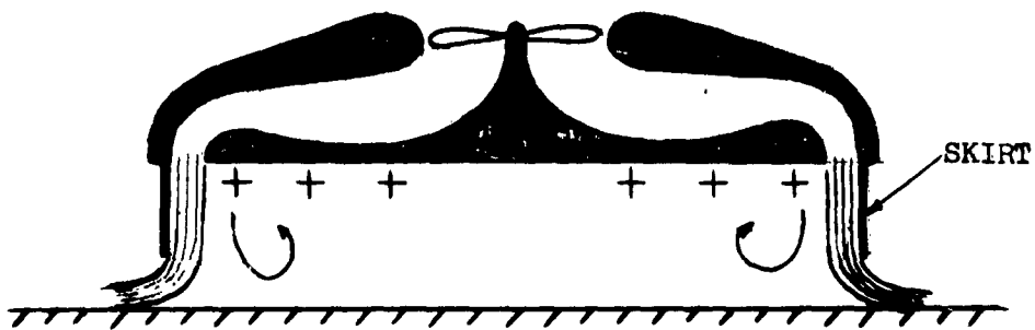
(a) ANNULAR JET WITH SKIRT
