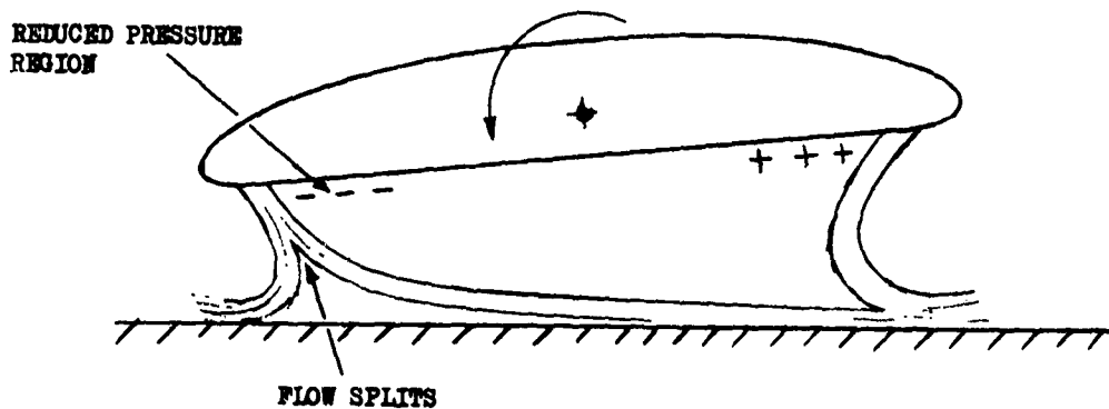
STATIC INSTABILITY OF SINGLE ANNULAR JET
