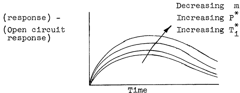
Figure 2 common for all P^* and T_1^* , and is the slowest response. Figure 3 shows qualitatively the differences between any response curve and the open circuit response curve.
