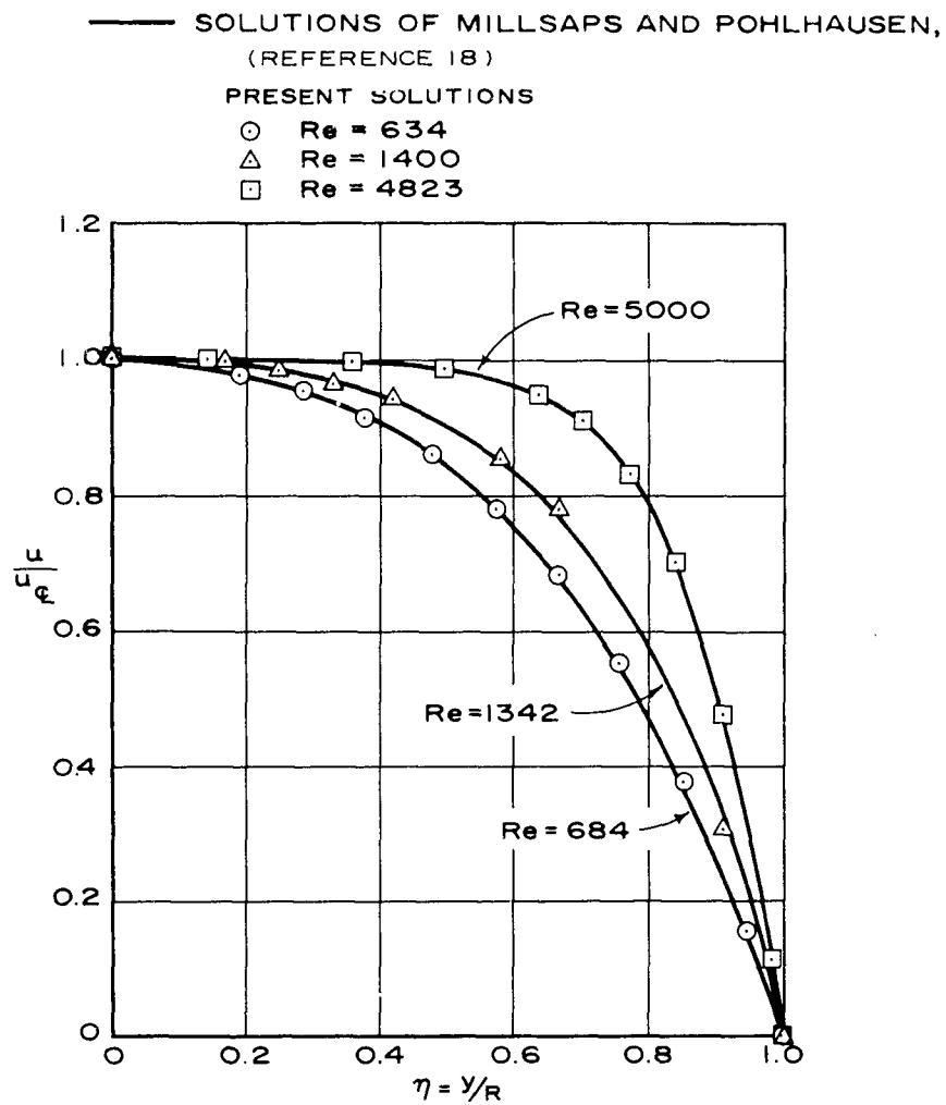
Figure 17 Convergent Channel With 5° Half Angle.
