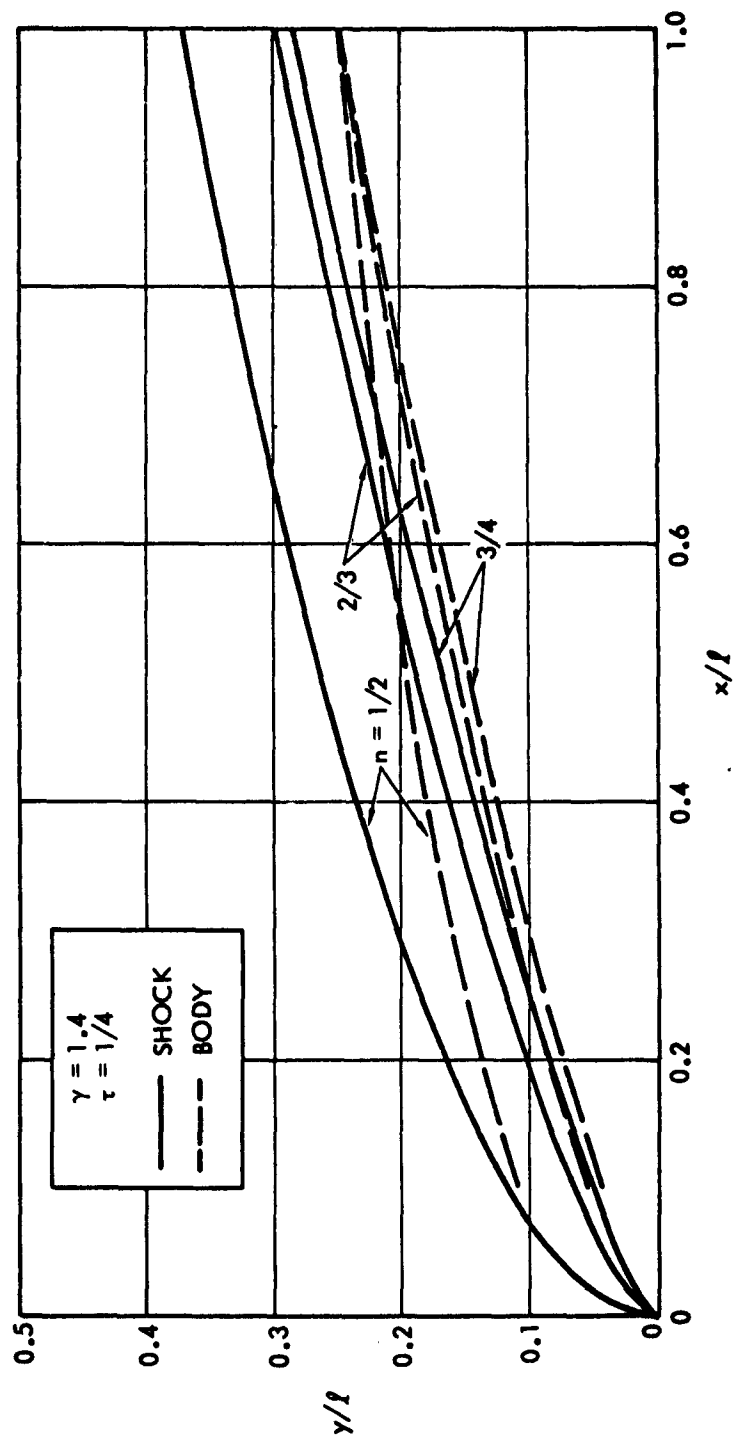
Figure 2. Bodies With Power-Law Shocks
