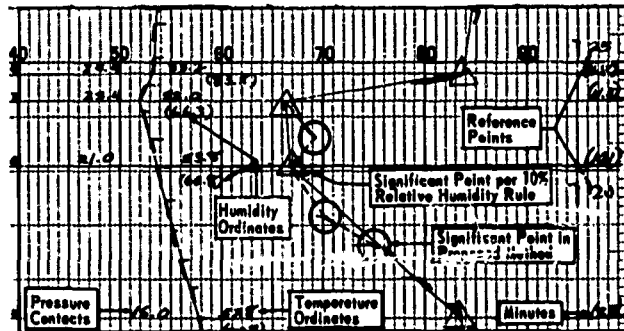
Fig. 6: Portion of Radiosonde Recorder Record, Eglin Main, 1700Z, 26 October 1962.
