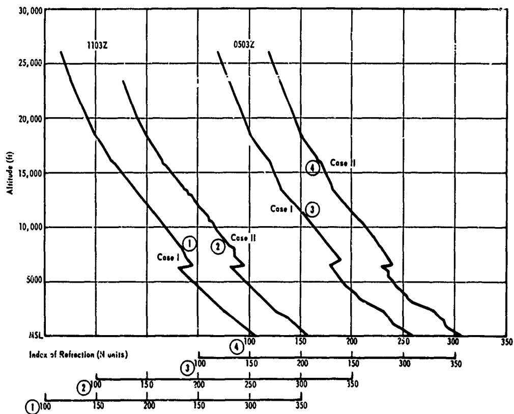
Fig. 9: Comparison of Electrical Index of Refraction Profiles Derived by the proposed Method and by the 10-Percent Relative Humidity Rule, Eglin Main, 0503Z and 1103Z, 13 February 1963.
