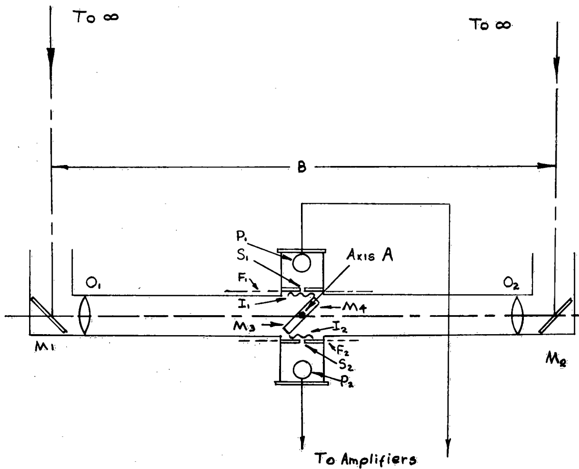
Figure 11. Construction of range-finder system when rotating double mirror is employed for scanning.
