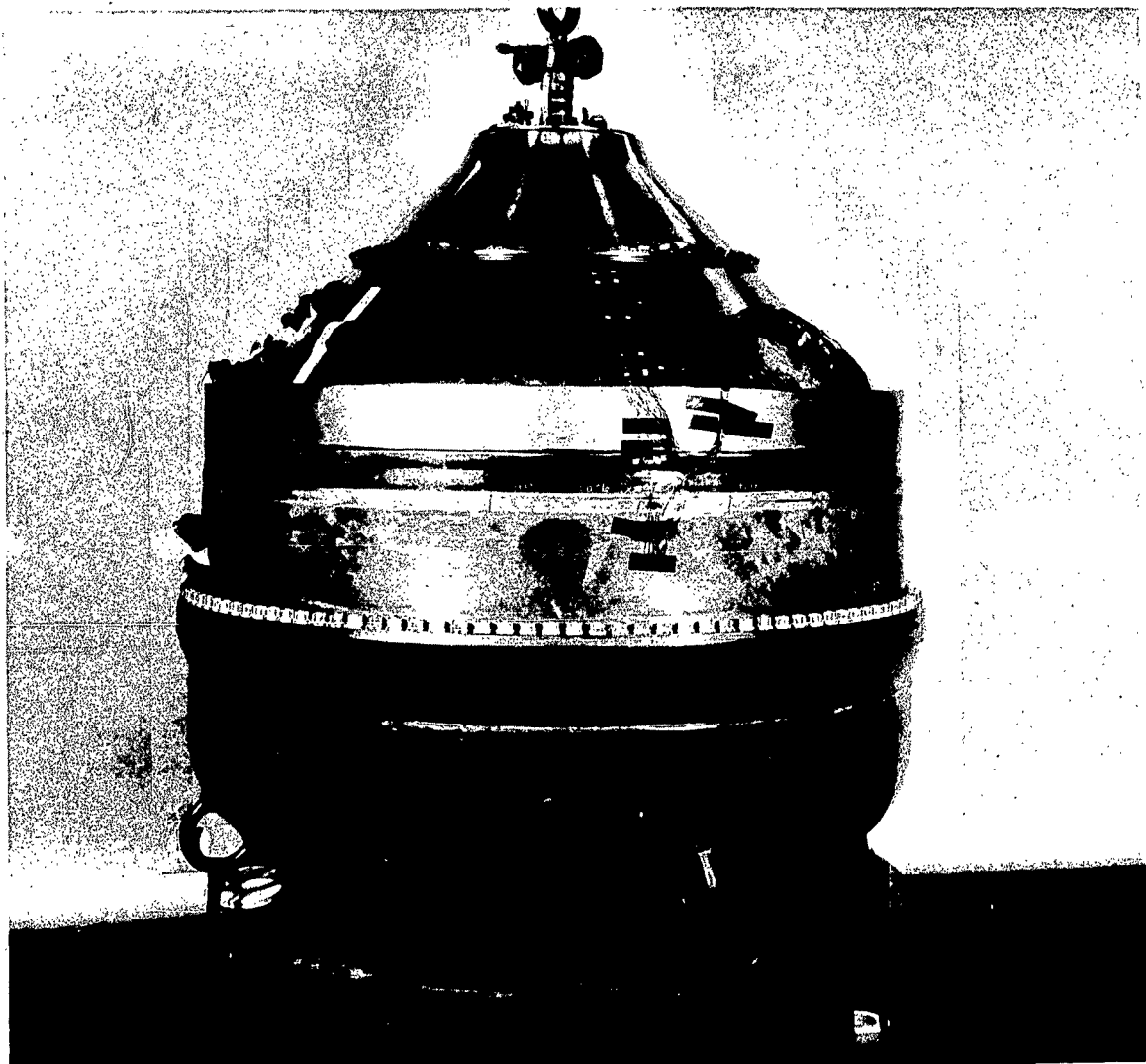
B-120 VCA TITANIUM 40-INCH DIAMETER REAR DOME COMPONENT ASSEMBLY FOR HYDROSTATIC TESTING
