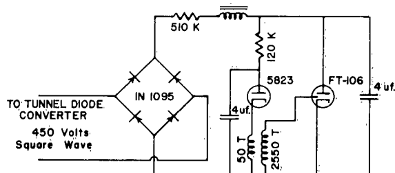
Fig. 3 - Flashing light circuit
