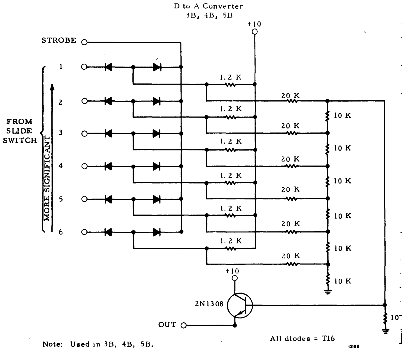
Figure I-13. Digital To Analog Converter
