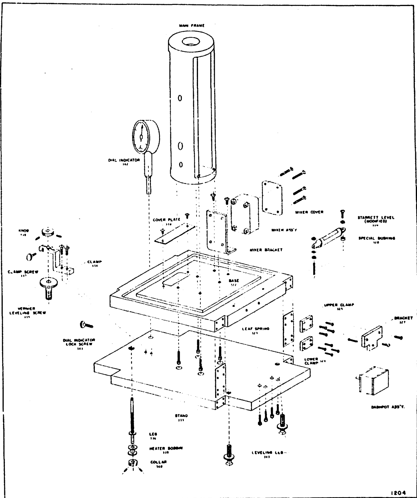
Figure 14. Base Assembly
