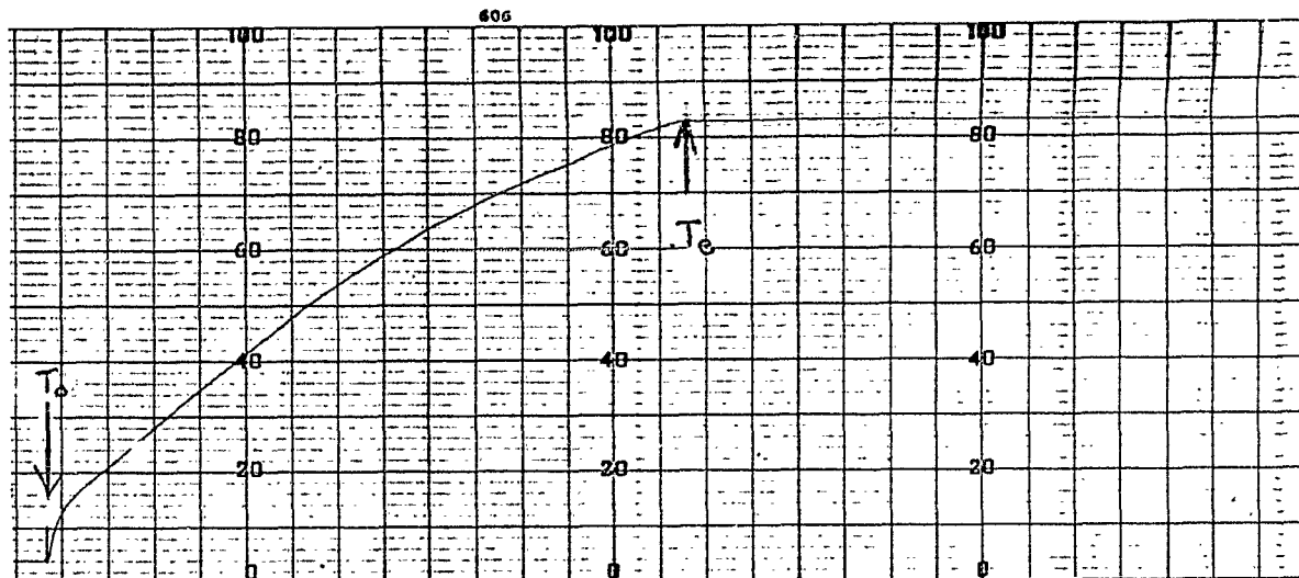
Fig. 25 TEST NO. 13, PLATE TEMPERATURE RISE TO 2000°F (Rise Rate T_o to T_e = 17.1^\circ\text{F}/\text{sec} )
