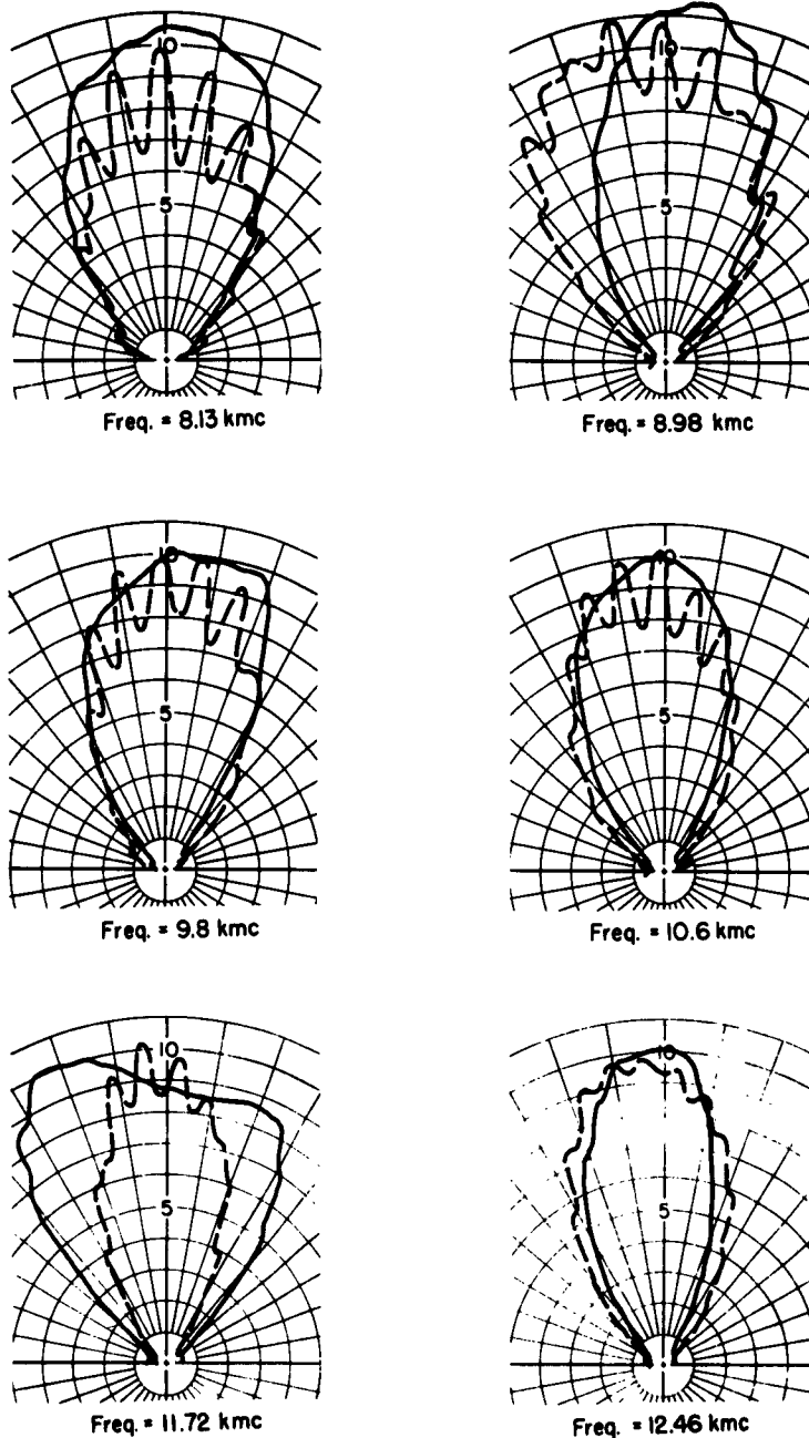
Fig. 10. Patterns in the plane orthogonal to the plane of tilt obtained with a 21^\circ wedge with a dielectric constant of 6 in a 3.75'' \times 0.81'' aperture fed by a 60^\circ flare sectoral horn. Polarization of solid patterns is normal to the plane of the pattern. Polarization of dashed patterns is in the plane of the pattern.
