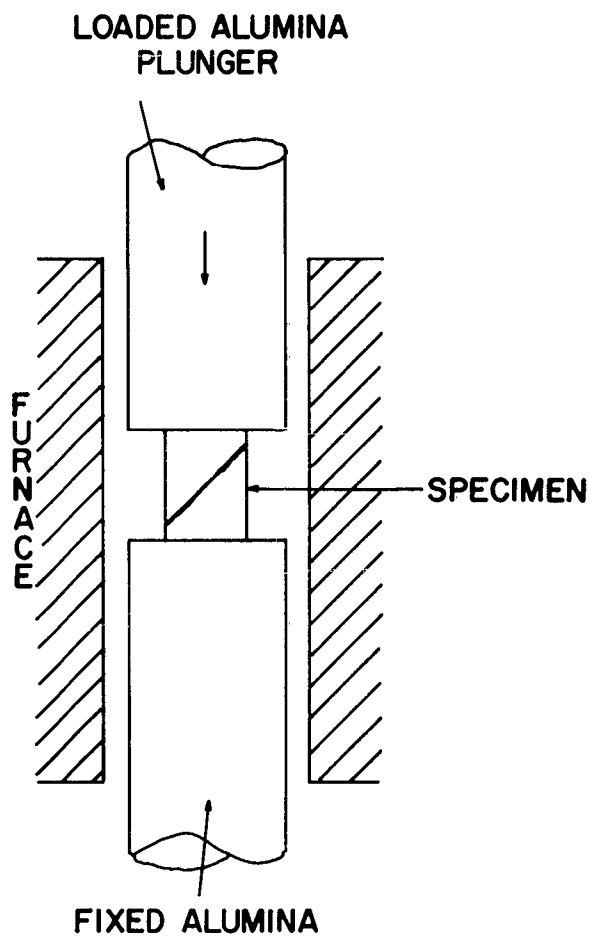
FIGURE 2. CREEP-RUPTURE TEST APPARATUS
