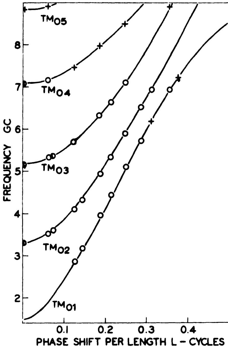
Fig. 2. A Brillouin diagram for Section J.
