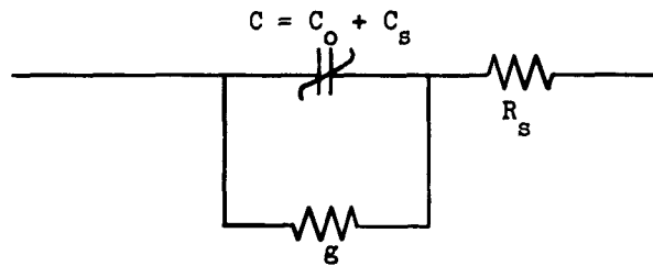
FIG. 4--Encased diode equivalent circuit.
