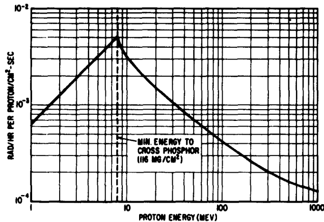
Fig. 4 - Absorbed dose rate per unit proton flux, averaged over the volume of \text{CaF}_2:\text{Mn} in a dosimeter. The dosimeters have an inner diameter of about 0.74 mm and are filled with phosphor powder to a density of 1.57 g/cm 3 , giving 0.116 g/cm 2 mass thickness across the diameter (see the text for additional details about the calculation).
