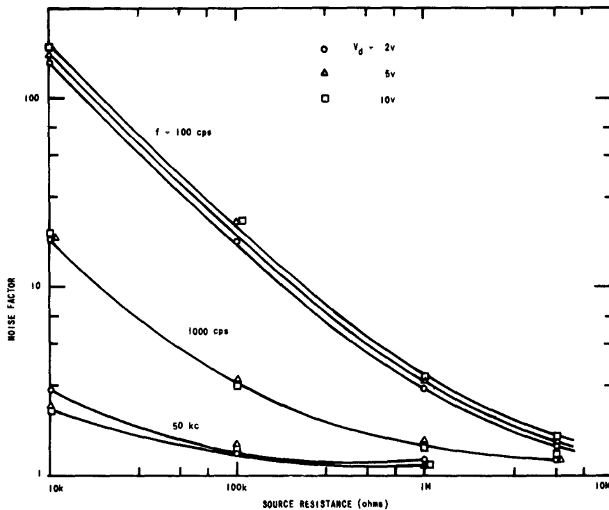
FIG. 40. NOISE FACTOR VS SOURCE RESISTANCE FOR DEVICE FSP400 WITH FREQUENCY AND DRAIN BIAS AS PARAMETERS ( V_g = 0 \text{ v} ).
