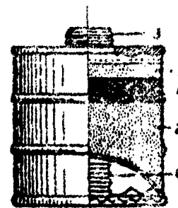
Fig. 6. Hopcalite cartridge: 1 - hopcalite 2 - desiccant layer 3 - threaded joint 4 - internal threaded joint.
