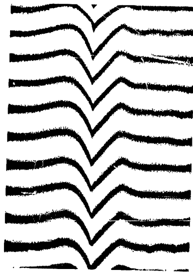
Figure 12. Surface of Sample 4. X865. Fringe spacing = 0.27 \mu .
