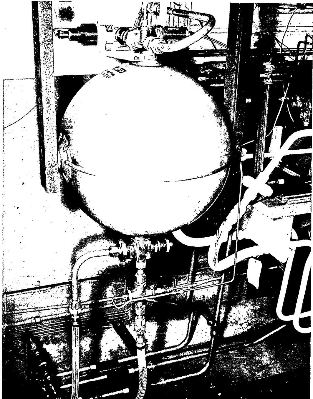
Figure 13. View of Long Ullage Fitting Test Setup, Showing Oxidizer Start Tank
