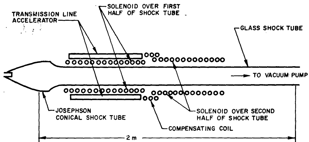
Fig. 4. Schematic of Apparatus
