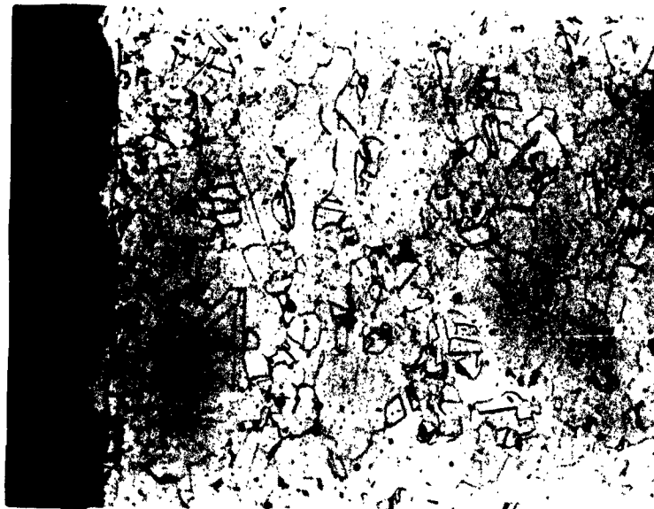
FIGURE 5 PHOTOMICRO GRAPHS OF INNER SURFACE OF NO. 2 CONTAINER 250X
