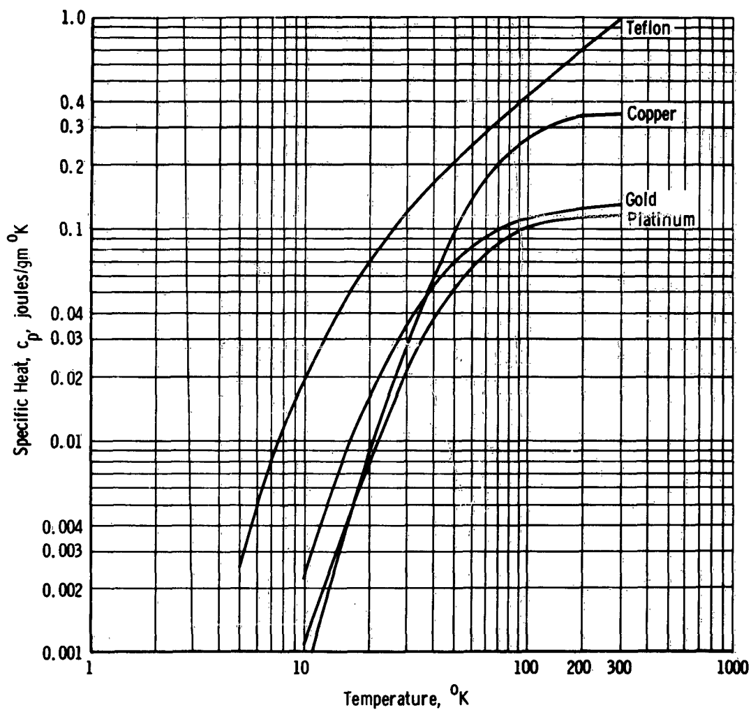
Fig. 24 Specific Heat vs Temperature
