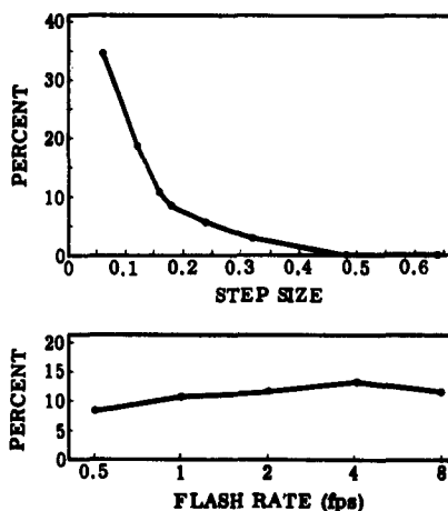
FIGURE 10. PERCENTAGE OF SUBPROBLEMS IN WHICH "ACCIDENTAL INITIAL CONVERGENCE" OCCURS, AS A FUNCTION OF STEP SIZE AND FLASH RATE
