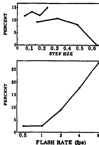
FIGURE 9. PERCENTAGE OF SUBPROBLEMS IN WHICH "NO CONVERGENCE" OCCURS, AS A FUNCTION OF STEP SIZE AND FLASH RATE. The small- and large-step problems are plotted separately, the small extending from 0.06 to 0.24 and the large from 0.16 to 0.64.
