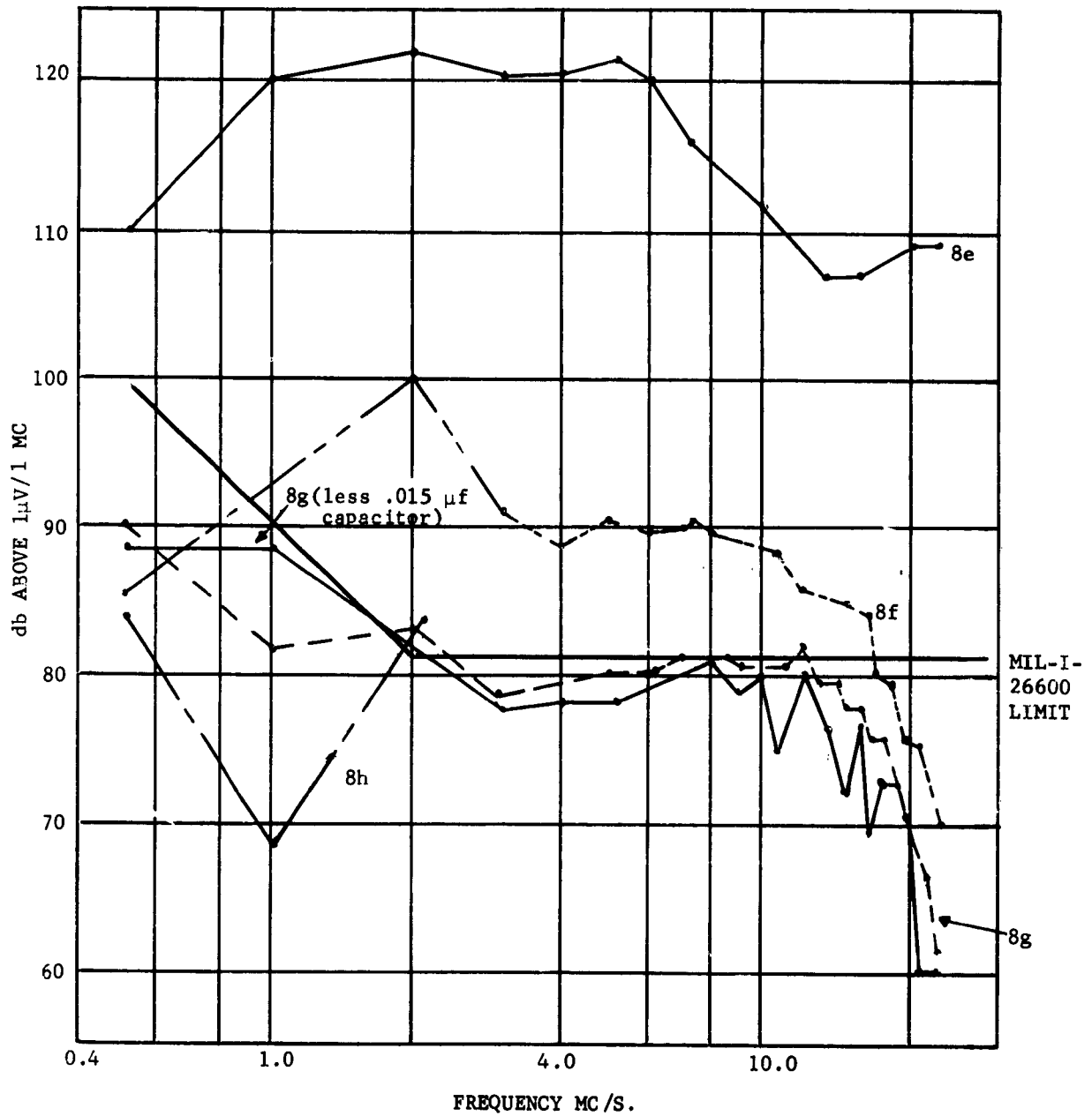
Figure 11. Conducted Interference Level of Bistable Multivibrator (Base Triggered)
