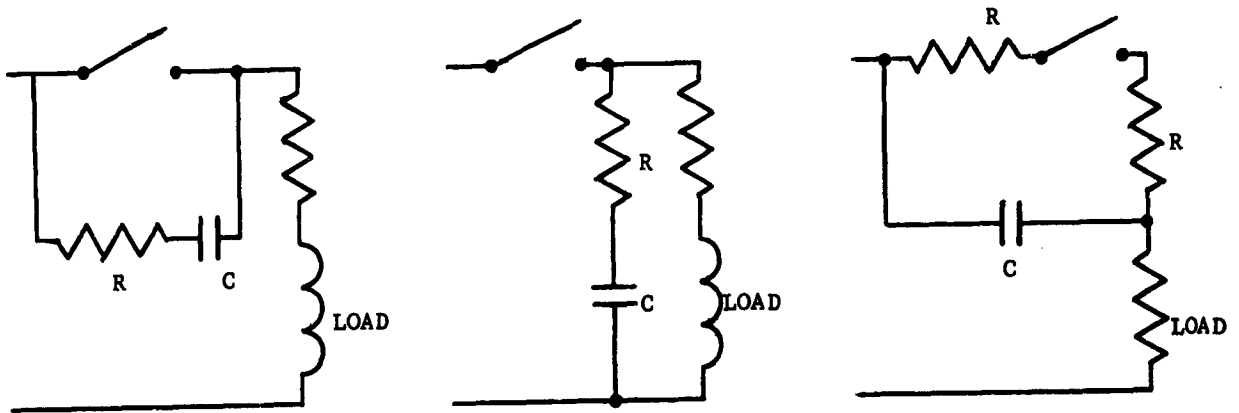
(c) R-C Suppression Elements
