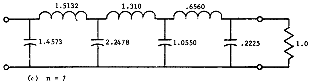
Figure II-3. Prototype Low-Pass Filters Having Butterworth Response
