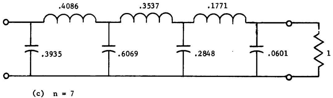
Figure II-5. Butterworth Filters with Values scaled to Provide 60 db Attenuation at Common Frequency
