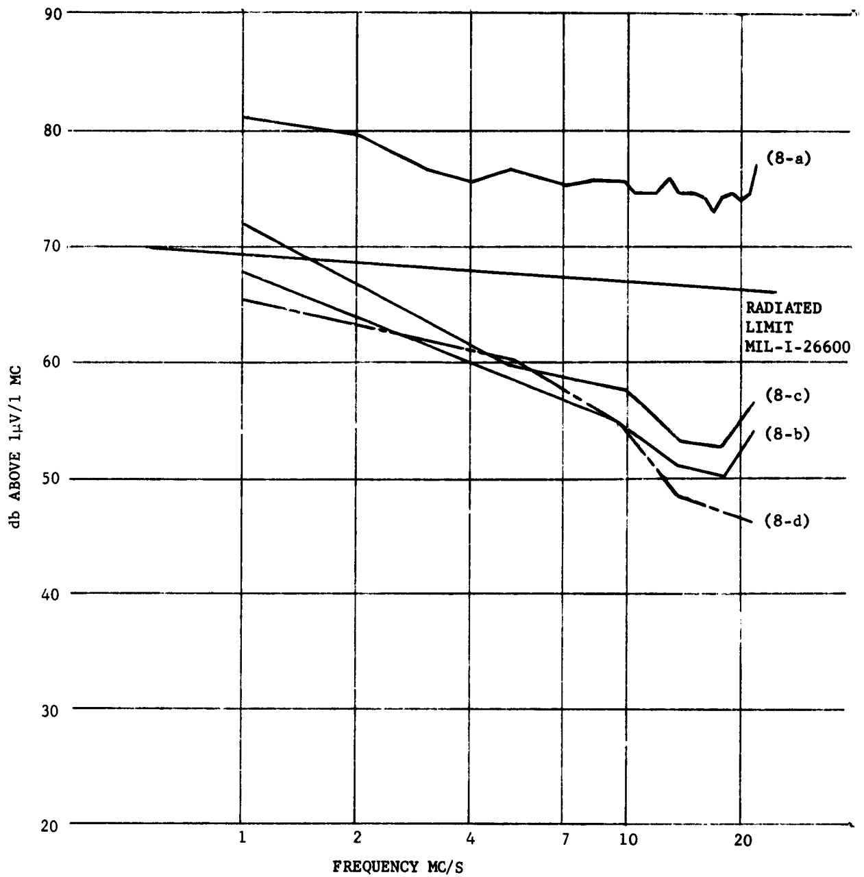
Figure 10. Radiated Levels from Power Supply Lines for Blocking Oscillator with Decoupling Filters of Figure 8.
