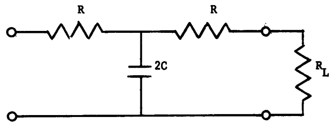
(c) Tee Section
