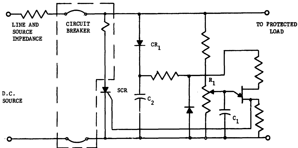
Figure 17. Littelfuse Transistor Protector
