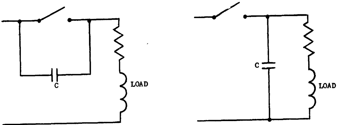
(b) Capacitor Suppression Elements
