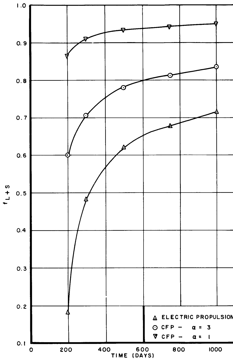
Figure 13. Comparison of CFP System with Electric System Based on Usable Payload: One-Way Trip to Jupiter
