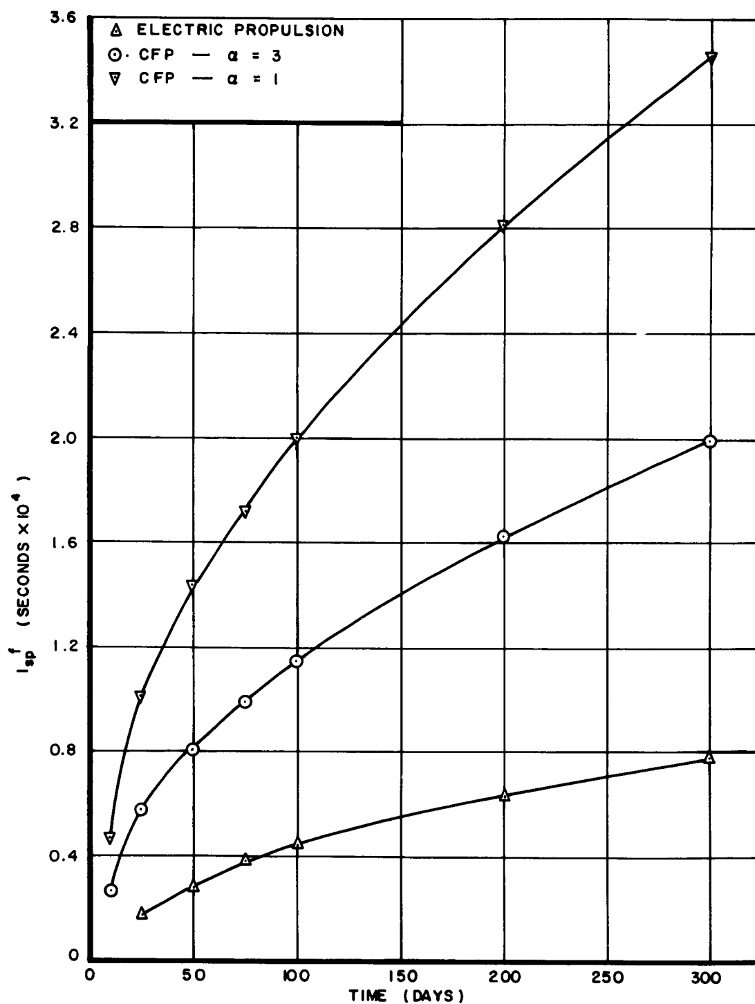
Figure 32. Comparison of CFP System with Electric System Based on Specific Impulse Used at Completion of Mission: Round Trip to Moon
