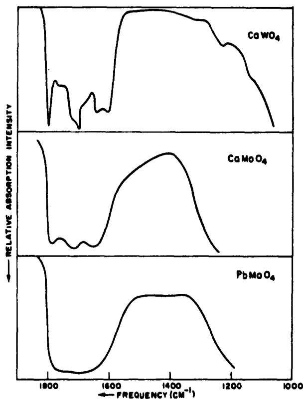
Fig. 7. The near infrared absorption spectra of \text{CaWO}_4 , \text{CaMoO}_4 , and \text{PbMoO}_4 at liquid nitrogen temperature.
