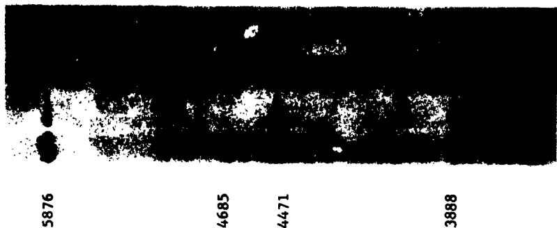
Fig. 47 Helium Broadening and Forbidden Transitions
