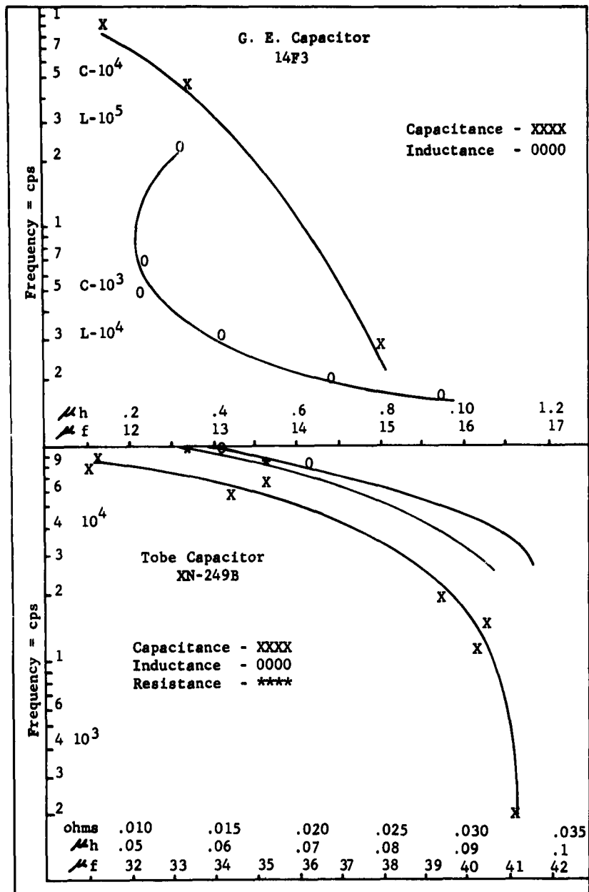
Fig. 1. Variation of Apparent Capacitor Characteristics with Frequency
