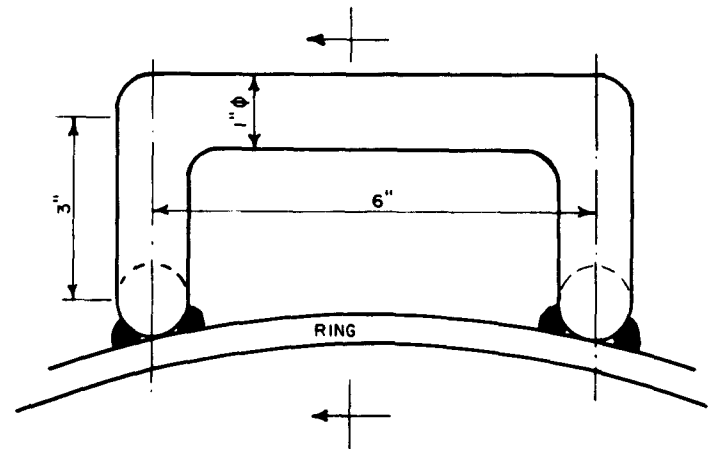
HANDLE DETAILS
