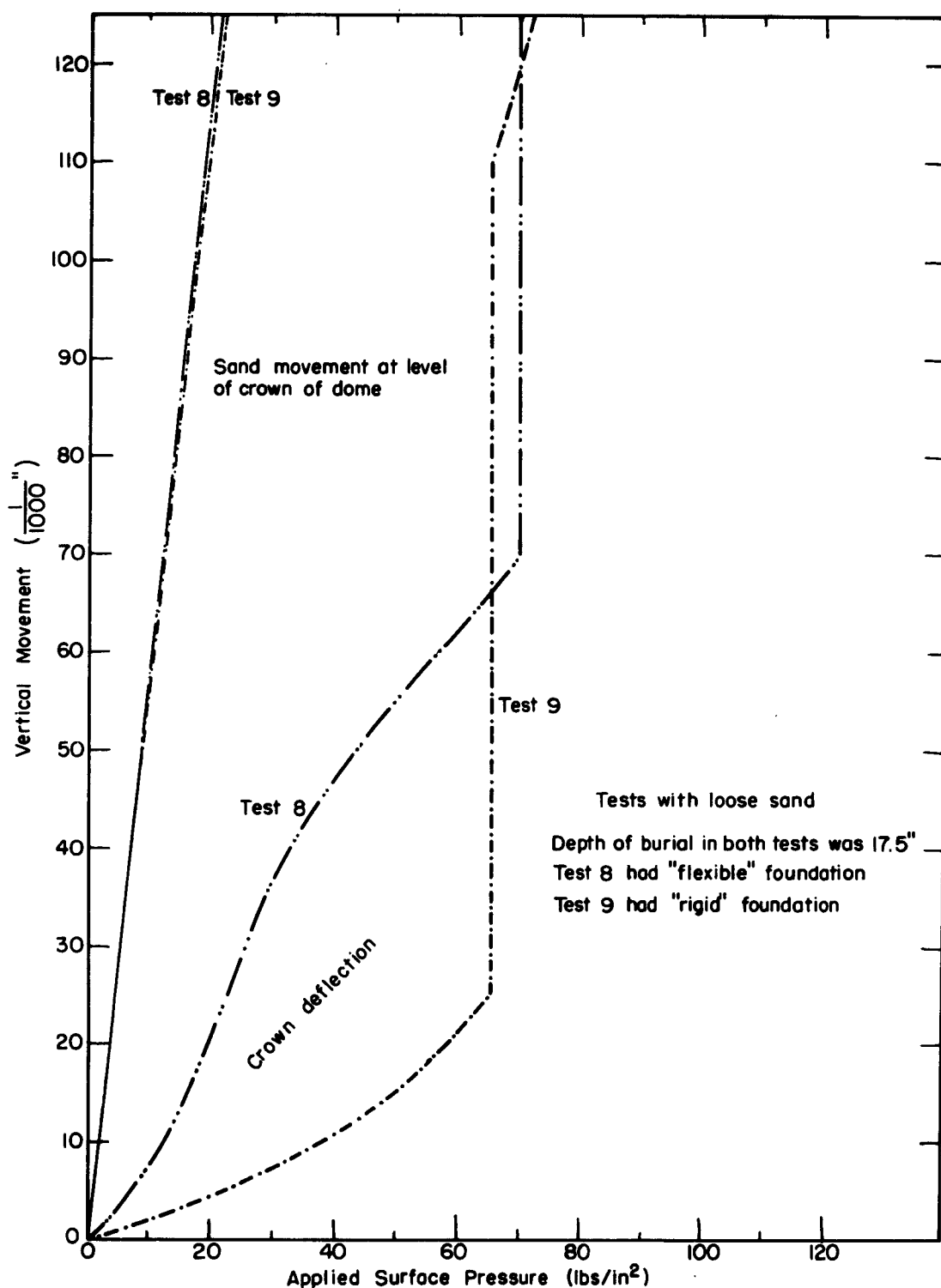
FIGURE E-36 COMPARISON BETWEEN CROWN DEFLECTION AND SAND MOVEMENT - TEST 8 & 9
