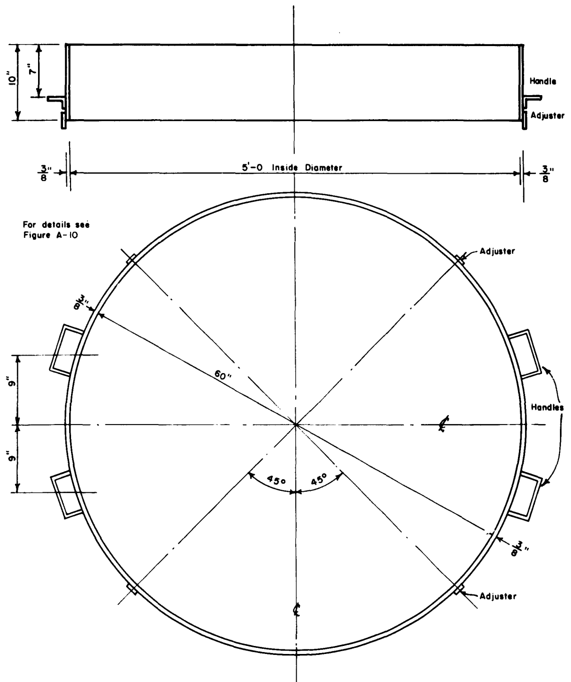
FIGURE A-8 STEEL BIN: RING DETAILS
