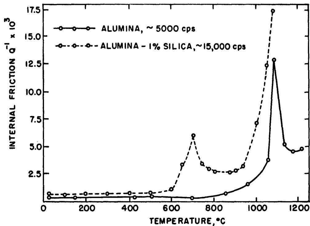
Figure 5 - Effect of impurity on the internal friction spectrum of polycrystalline alumina. The addition of 1% \text{SiO}_2 introduces a new low temperature internal friction peak. (After Crandall et al (22) ).
