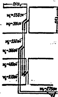
Diagram of one section of the \text{CFD}_4^4\text{PH} antenna
