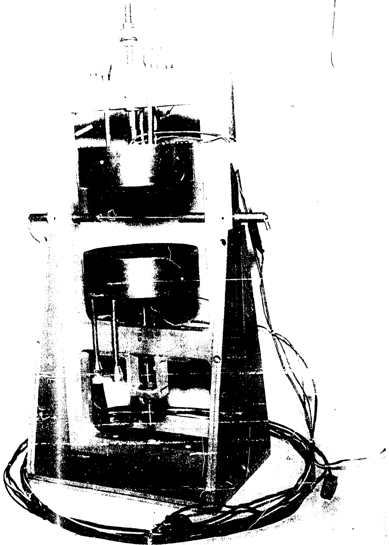
FIGURE 1. GAS VELOCITY MEASURING DEVICE
