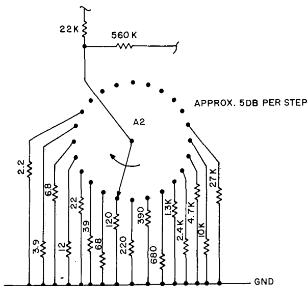
FIG.D-1 SCHEMATIC WIRING DIAGRAM OF TIMES FAX RECEIVER D-3
