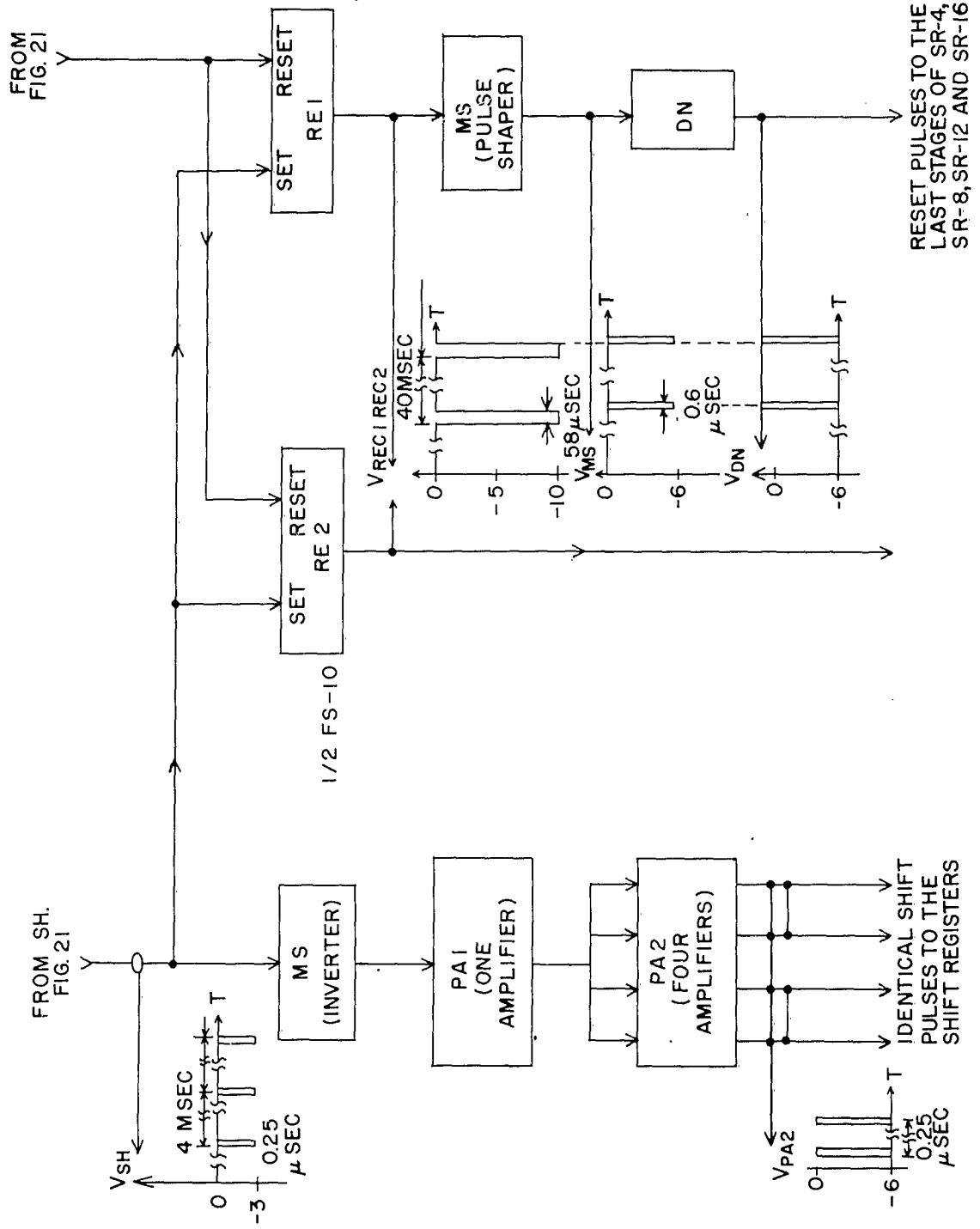
FIG.E-7 SPROCKET PULSE CIRCUIT
