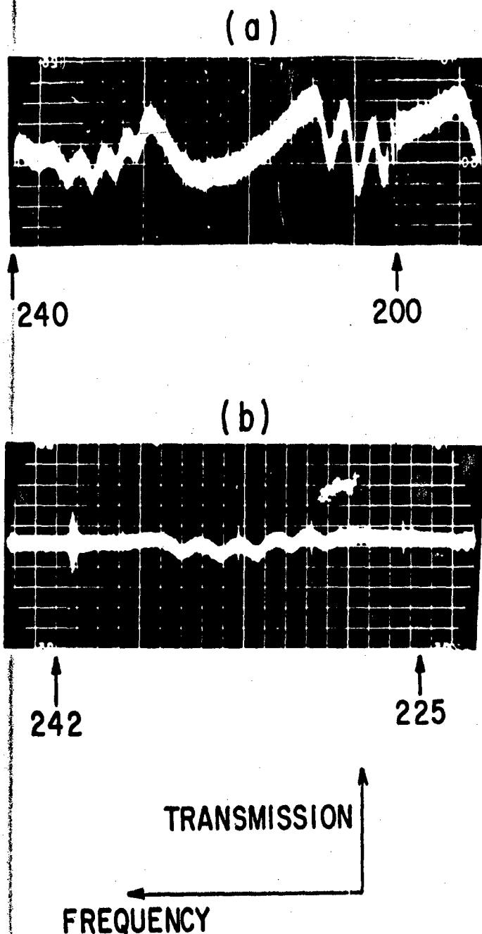
Fig. 5 Nuclear resonance absorption of MnAs and MnSb at 77°K: (a) MnAs showing absorption due to both Mn^{55} and As^{75} ; (b) MnSb showing absorption due to Mn^{55} . The frequency is given in Mc/s.
