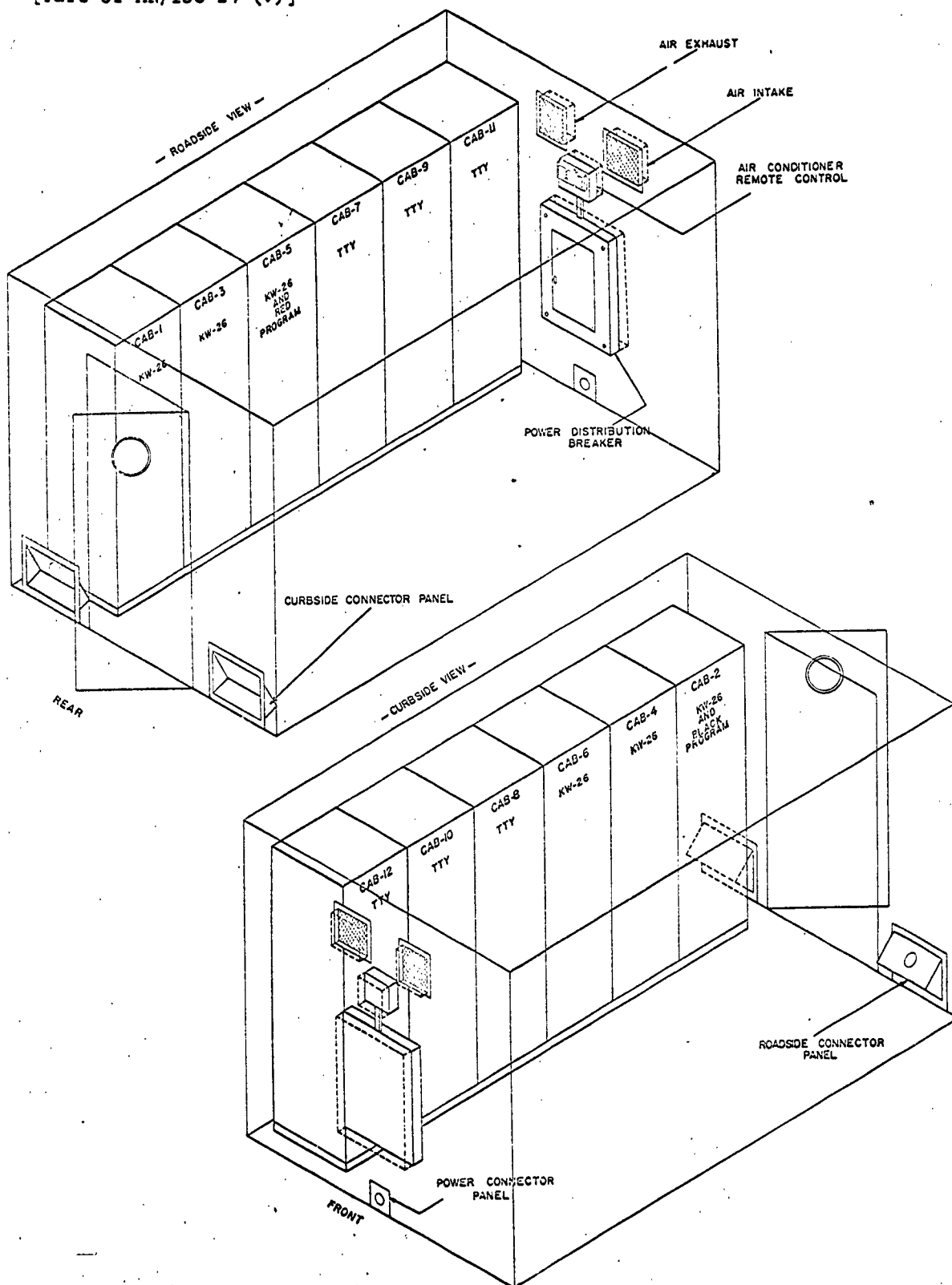
Figure 5 Equipment Layout, Relay Shelter
