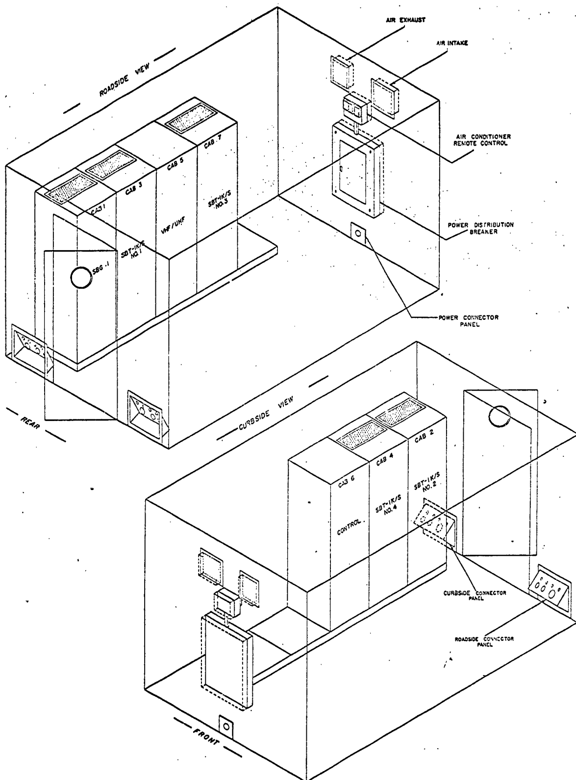
Figure 3 Equipment Layout, Medium Power Shelter (Sheet 24 of 99)
