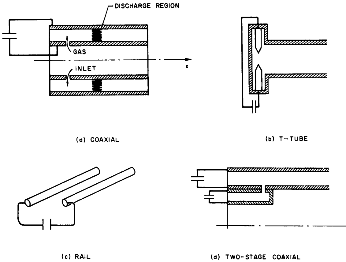
Fig. 1. Some Typical Geometries of Pulsed Plasma Accelerators
