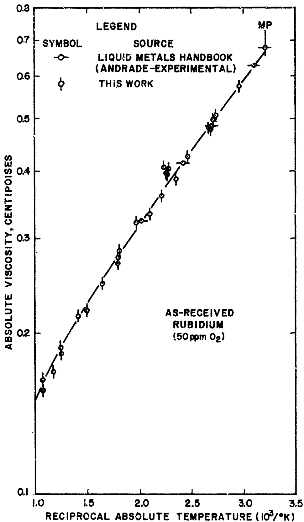
FIGURE 31. EXPERIMENTAL ABSOLUTE VISCOSITY DATA FOR AS-RECEIVED RUBIDIUM
