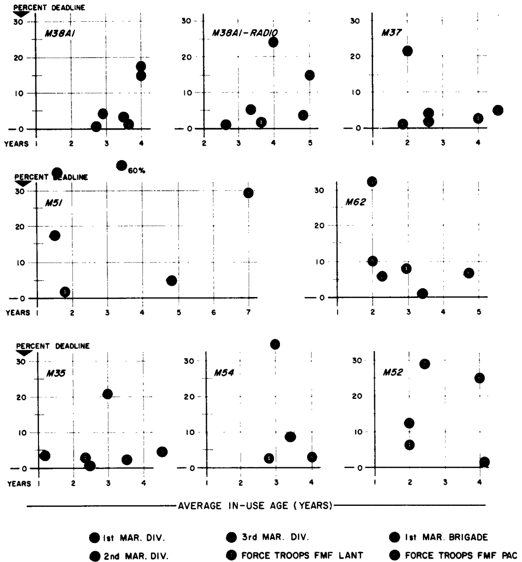
FIG. 6 AVERAGE PERCENT DEADLINE vs. AVERAGE IN-USE AGE FOR EIGHT TACTICAL VEHICLE TYPES
