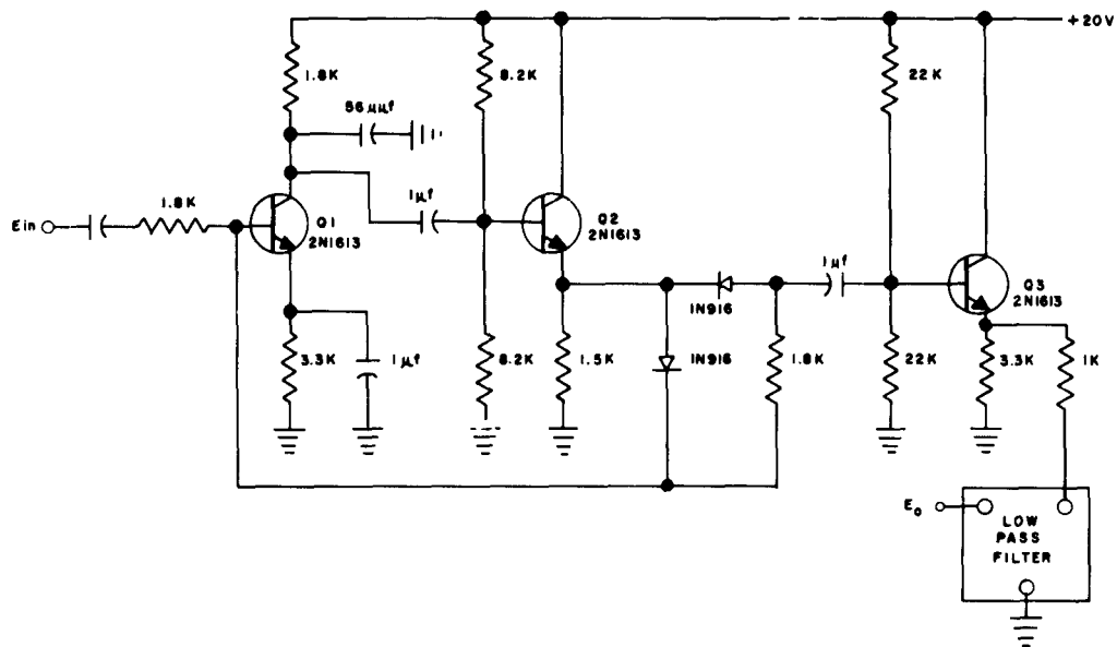
Figure 3. Envelope Detector Schematic
