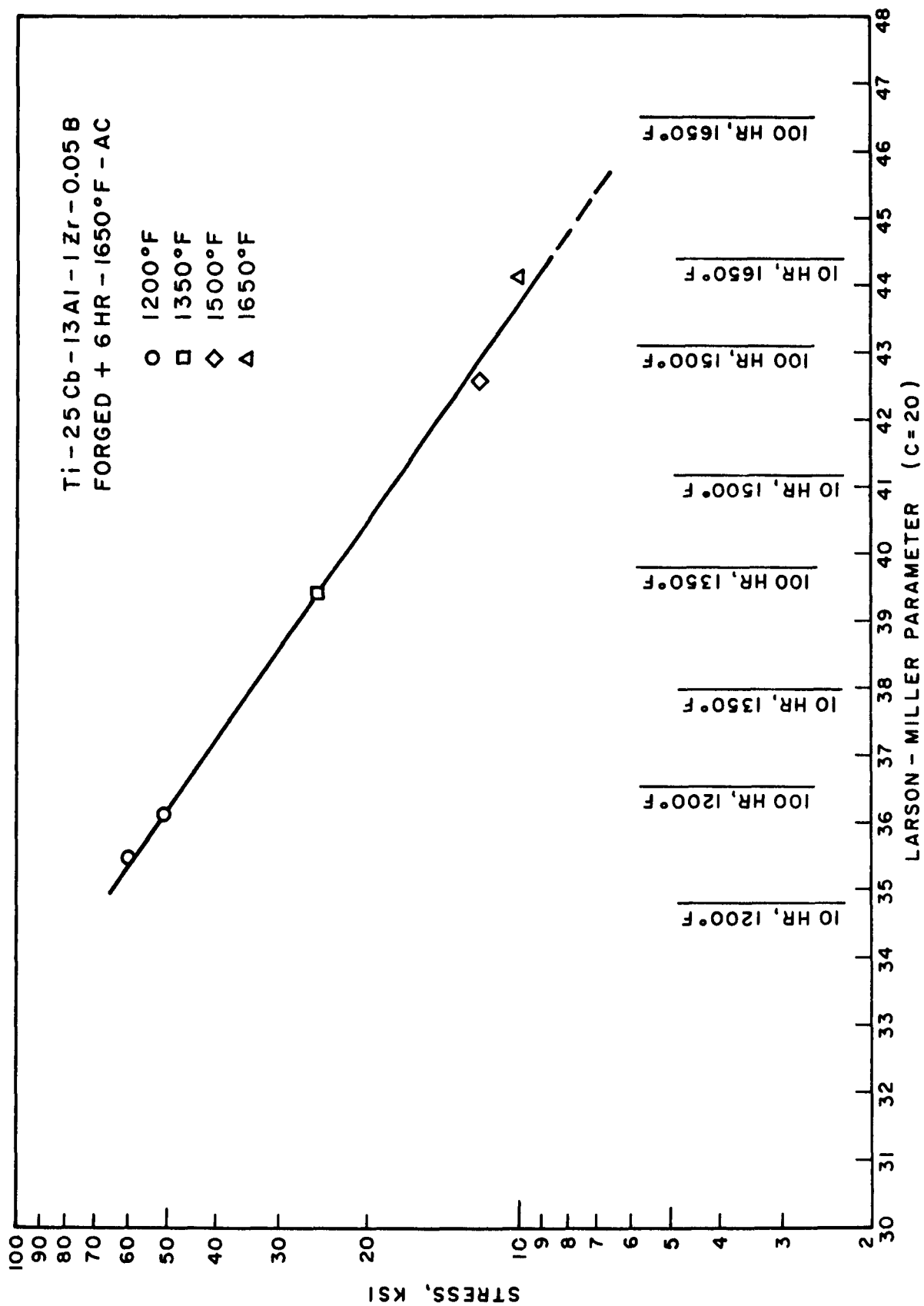
FIG. 15 - STRESS RUPTURE DATA FOR Ti-25Cb-13Al-1Zr-0.05B.
