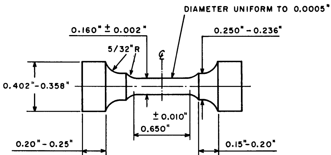
FIG. 1 HOUNSFIELD TENSILE TEST PIECE.
