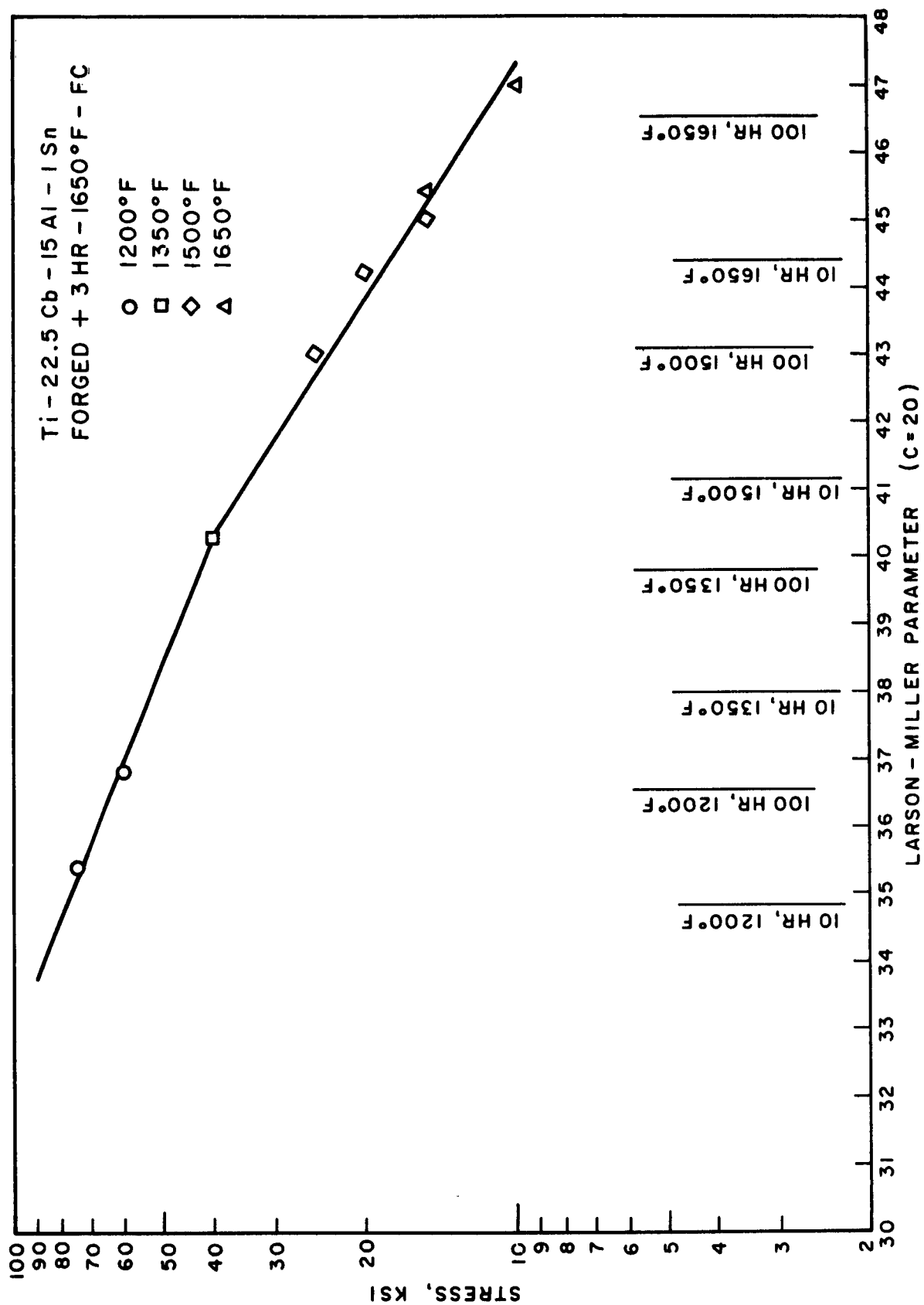
FIG. 9 - STRESS RUPTURE DATA FOR Ti-22.5Cb-15Al-1Sn.
