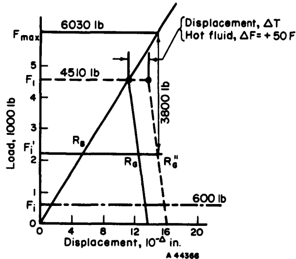
FIGURE 25. PRELOAD DIAGRAM FOR PLUS TEMPERATURE GRADIENT
