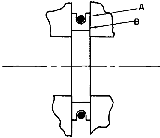
FIGURE 51. EXTERNAL-EXPLOSIVE SEAL
