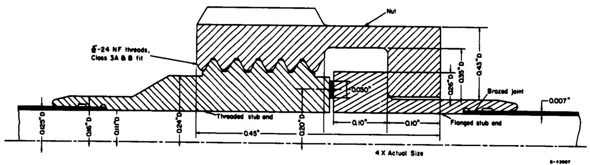
FIGURE 26. PROPOSED 1/8-IN. CLASS IIIa THREADED FITTING, 10,000 PSI AT -425 TO 600 F, RENÉ 41
