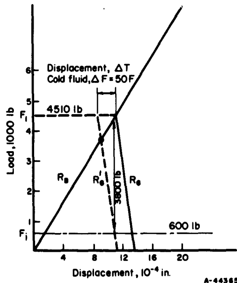
FIGURE 24. PRELOAD DIAGRAM FOR MINUS TEMPERATURE GRADIENT
