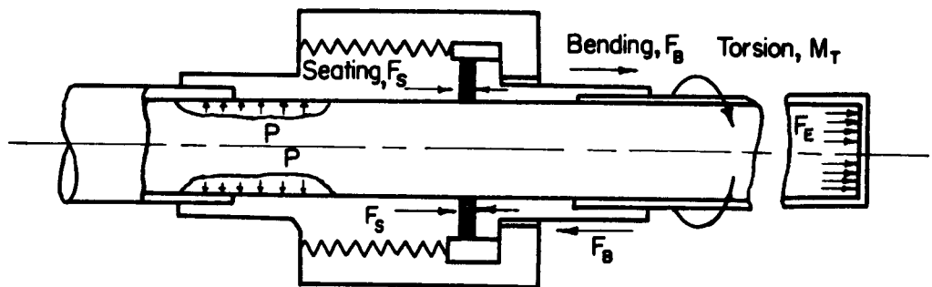
FIGURE 9. TYPICAL LOADS IMPOSED ON FITTINGS
