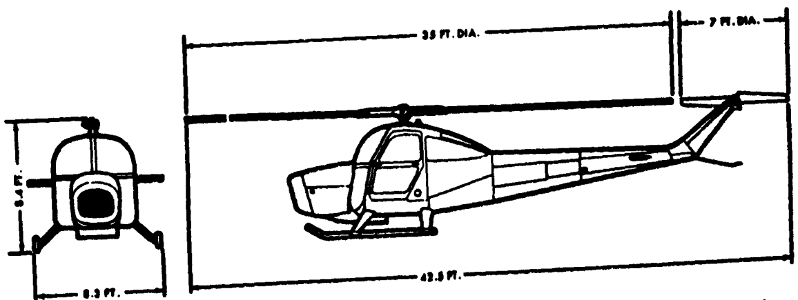
FIGURE 1. TEST HELICOPTER, U. S. ARMY YH-41 (MODIFIED), S/N 56-4236.
