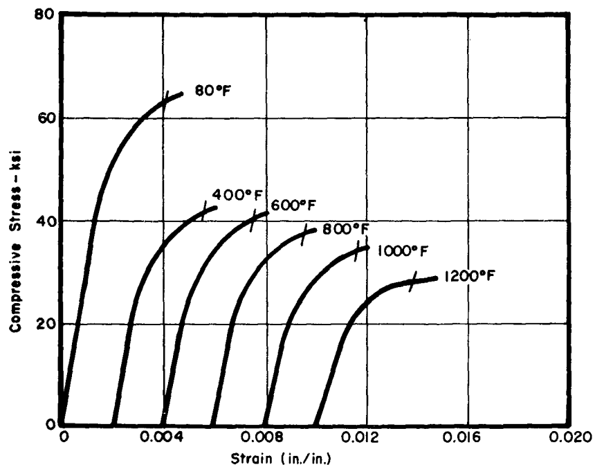
Figure 66. Compression Stress-Strain Curves of AM-350
