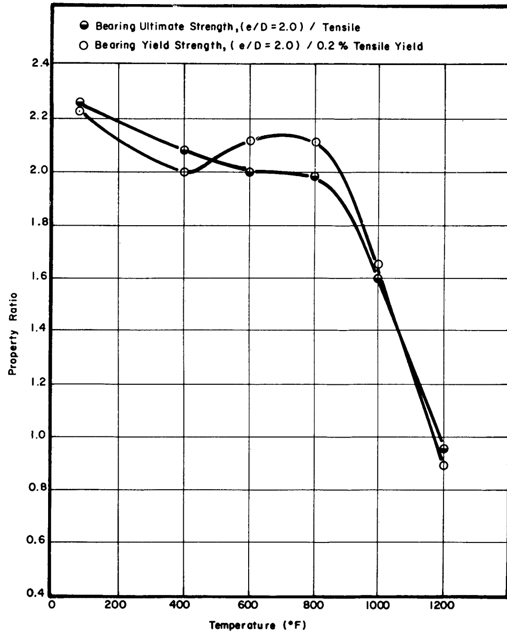
Figure 54. Effect of Temperature Versus the Bearing Properties/Tensile Properties of Potomac M, e/D = 2.0
