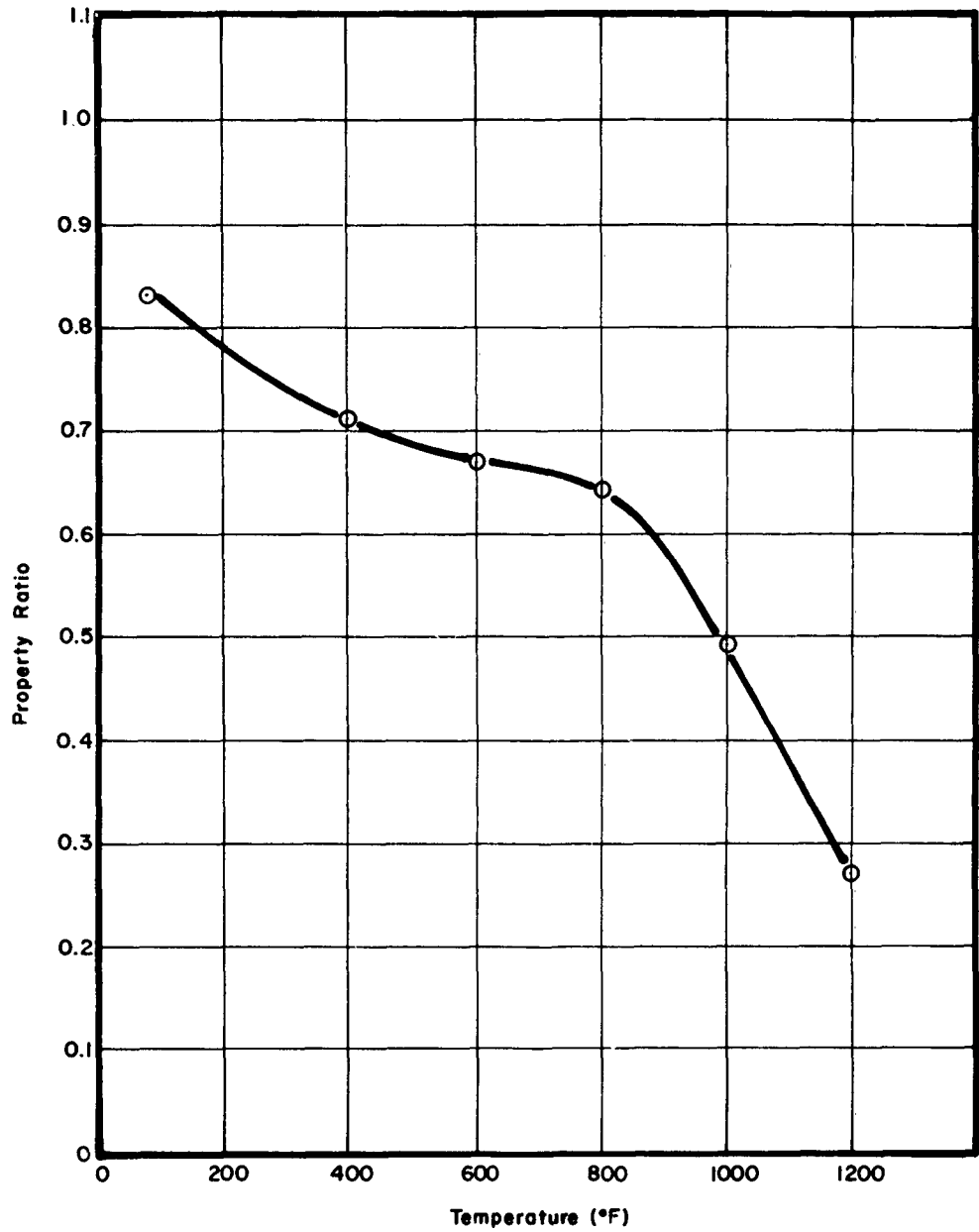
Figure 49. Effect of Temperature Versus the Sheet Shear Strength/Ultimate Tensile Strength of Potomac A
