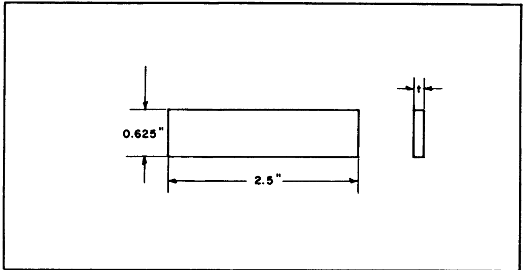
Figure 2. Compression Specimen
