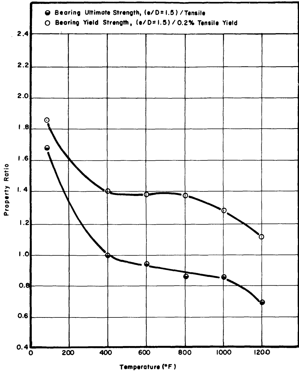
Figure 59. Effect of Temperature Versus the Bearing Properties/Tensile Properties of AM-350, e/D = 1.5
