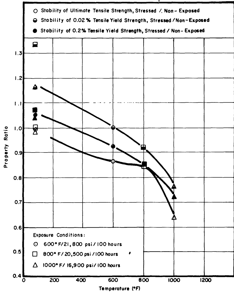
Figure 42. Effect of Exposure Time and Temperature Versus Stressed Tensile Stability/Tensile Properties of Non-Exposed Potomac M
