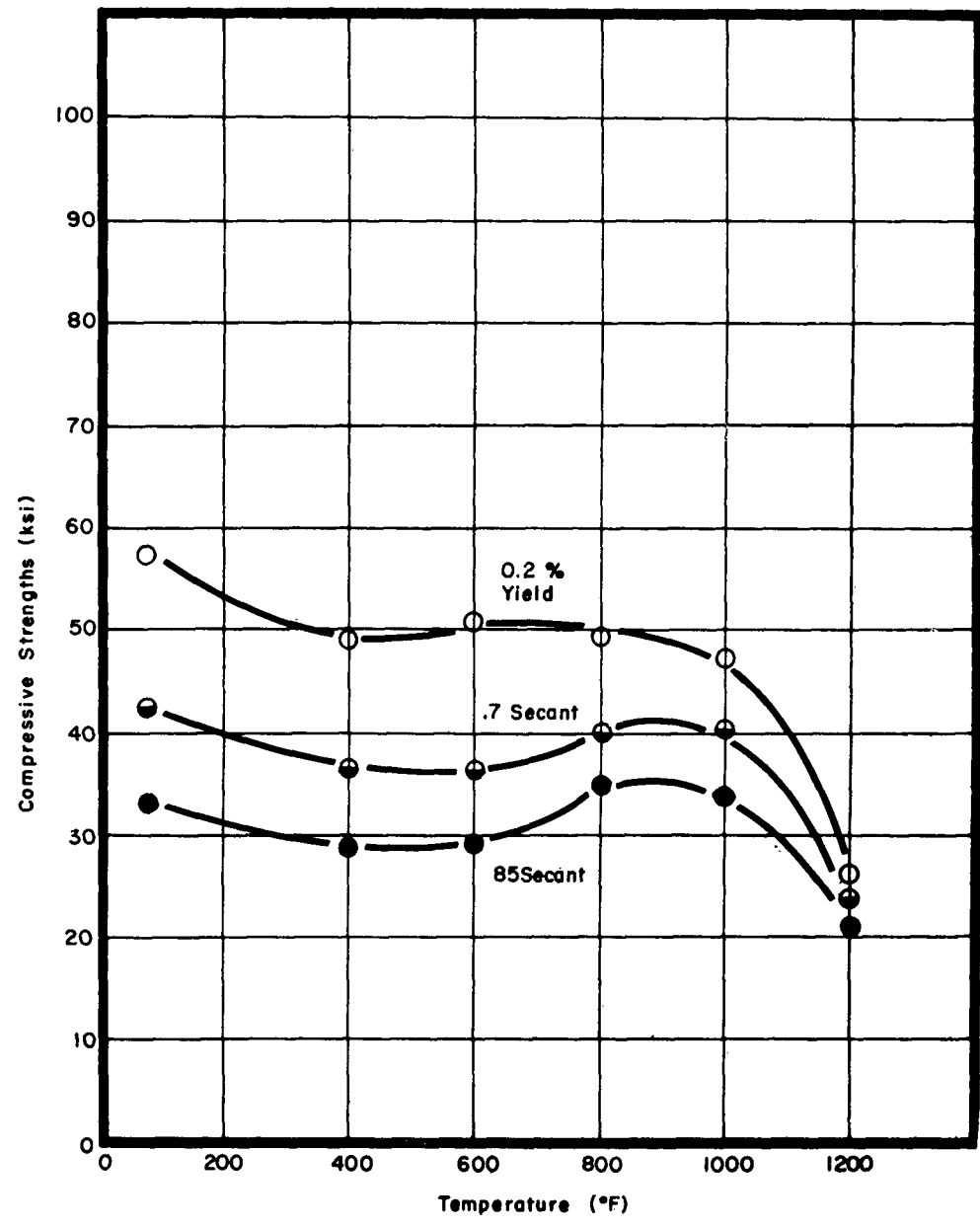
Figure 12. Effect of Temperature on Compressive Properties of Potomac A
